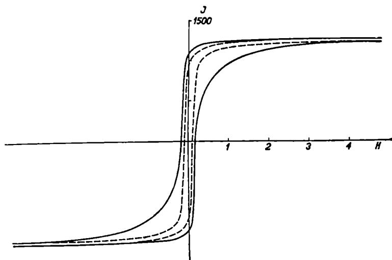
Fig. 42. Main loop of sample No. 3 (cf. Fig. 41).
