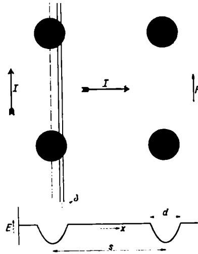
Fig. 1 Inclusion model of ferromagnetic hysteresis.
