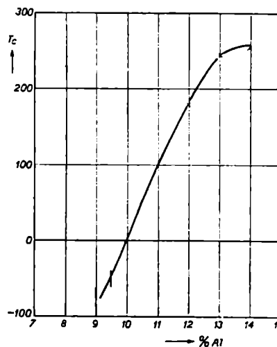
Fig. 35. The variation of the Curie temperature of the \epsilon -phase with aluminium content.
