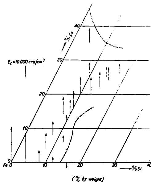
Fig. 8. E_c in the ternary system Fe-Co-Si .
