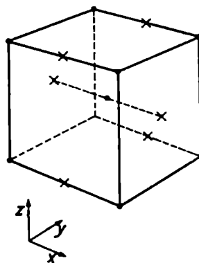
Fig. 15. Possible locations of C and N (H) atoms in the lattice of \alpha iron ( x -positions).
