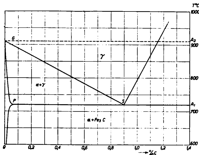
Fig. 50 Part of the iron carbon diagram.
