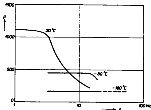
Fig. 29. Curves for \mu_0 for Cu Zn ferrite at three temperatures and at various frequencies.
