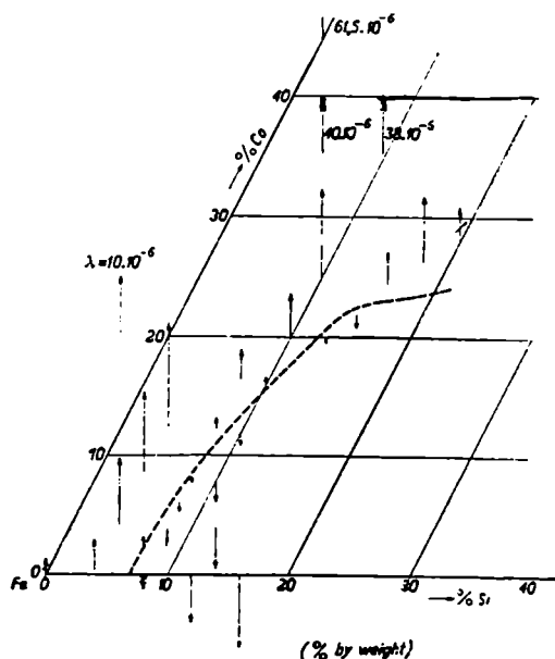
Fig. 7. \lambda in the ternary system Fe-Co-Si .
