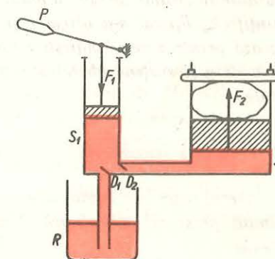
Fig. 2.110. Schema preseii hidraulice.
