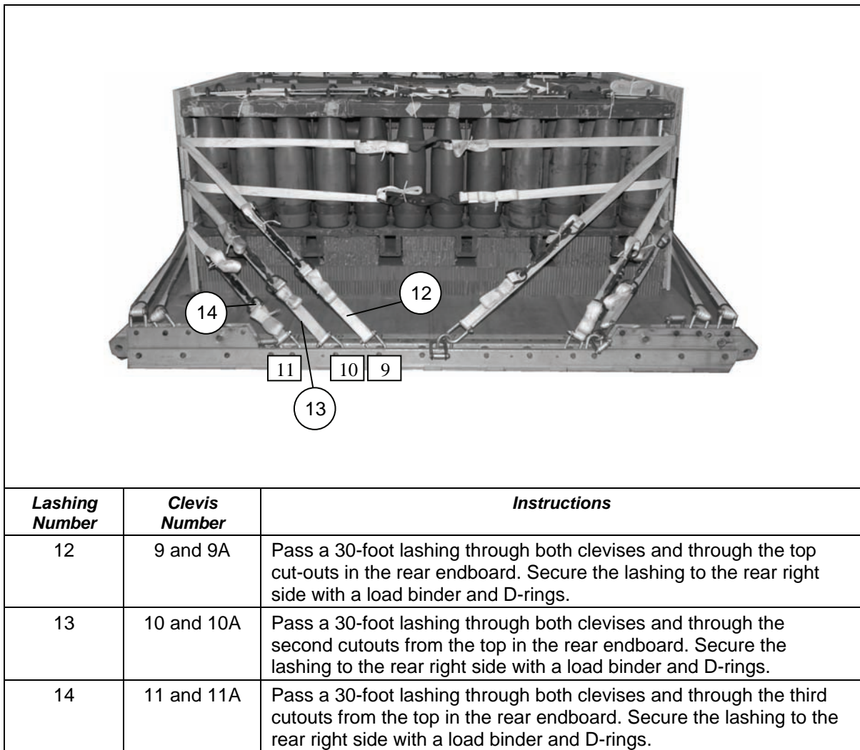
Figure 8-8. Ammunition Stack and Endboards Lashed (Continued)
