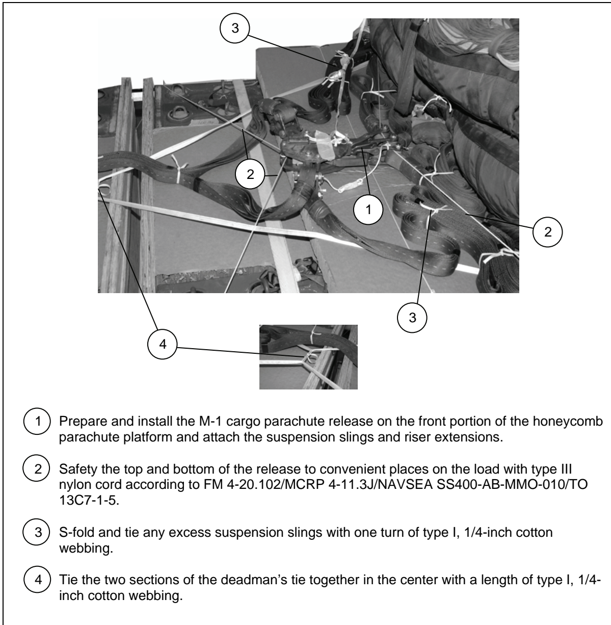
Figure 8-39. M-1 Cargo Parachute Release Installed
