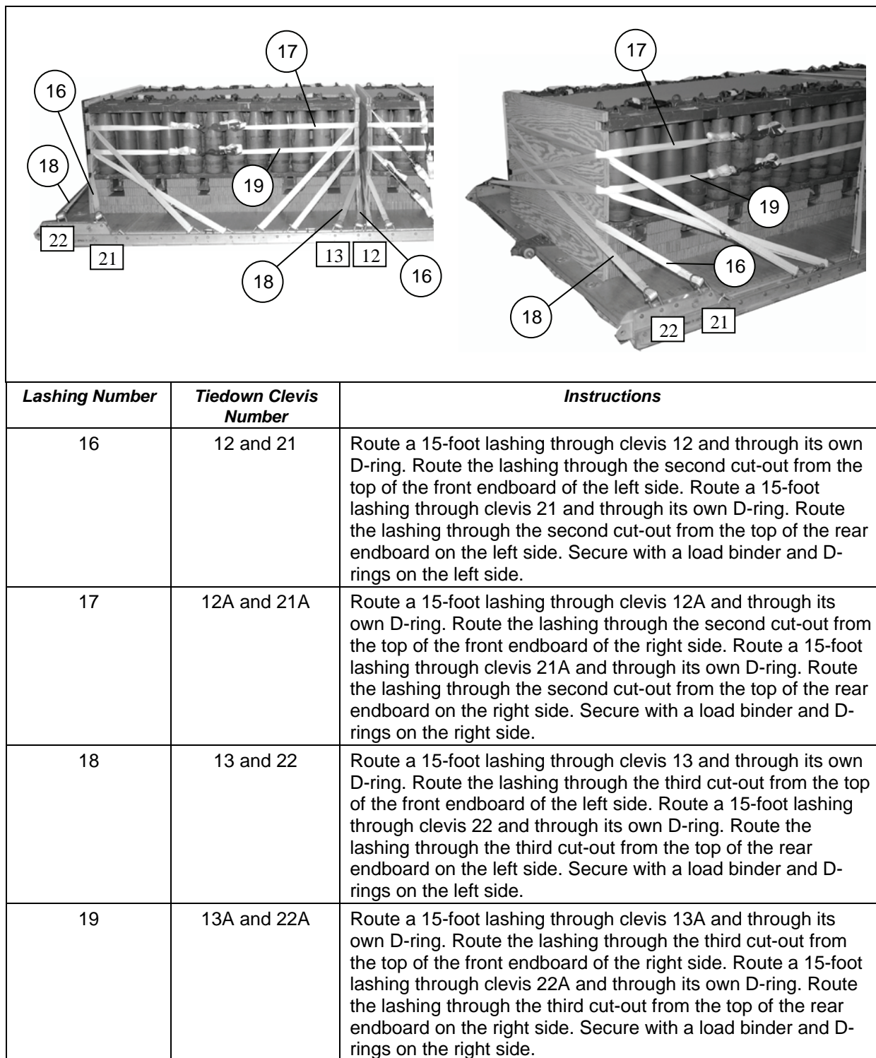
Figure 8-35. Second Ammunition Stack Lashed Using the Third and Fourth Endboards (Continued)
