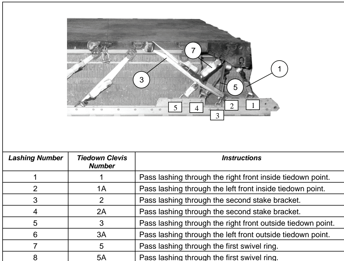
Figure 7-29. Pallet Lashed to Platform
