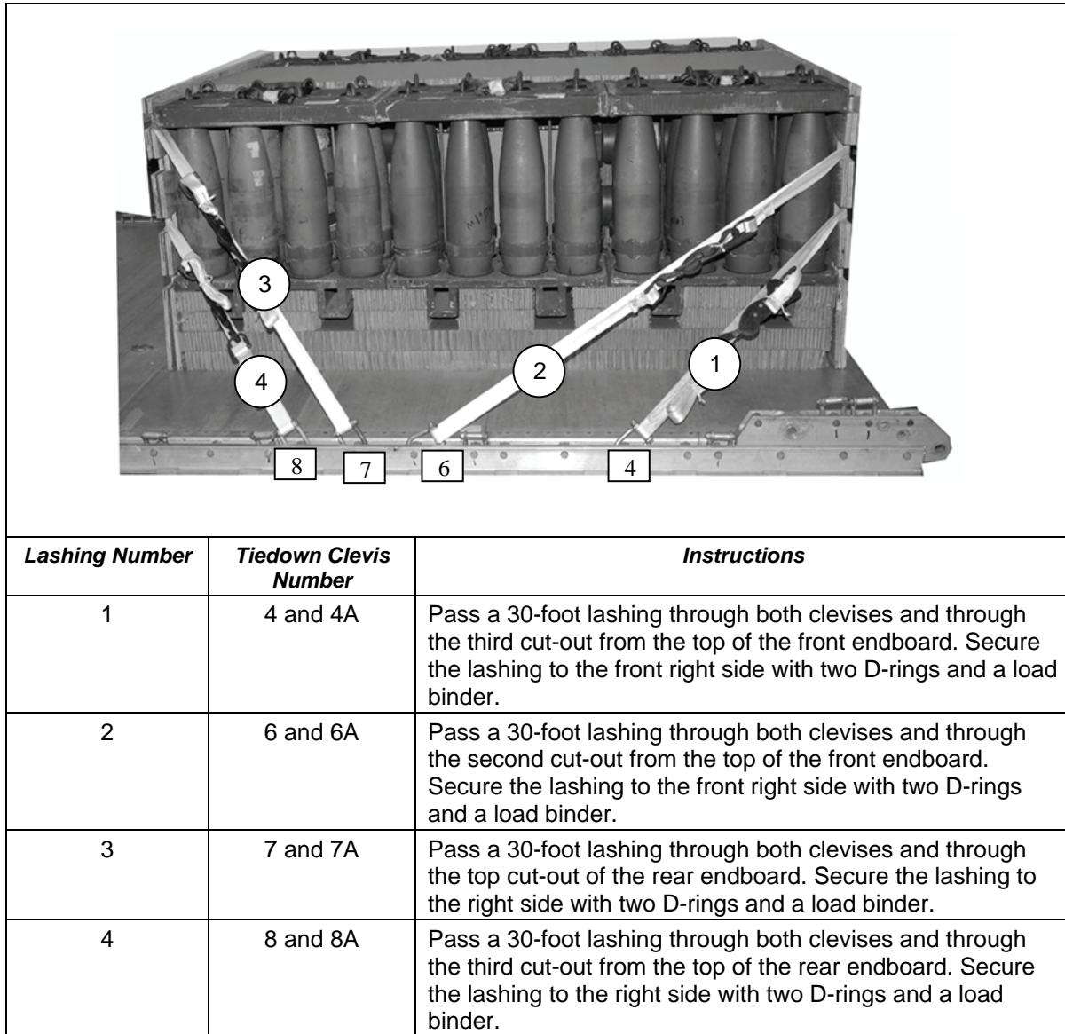
Figure 8-33. First Ammunition Stack Lashed Using the First and Second Endboards
