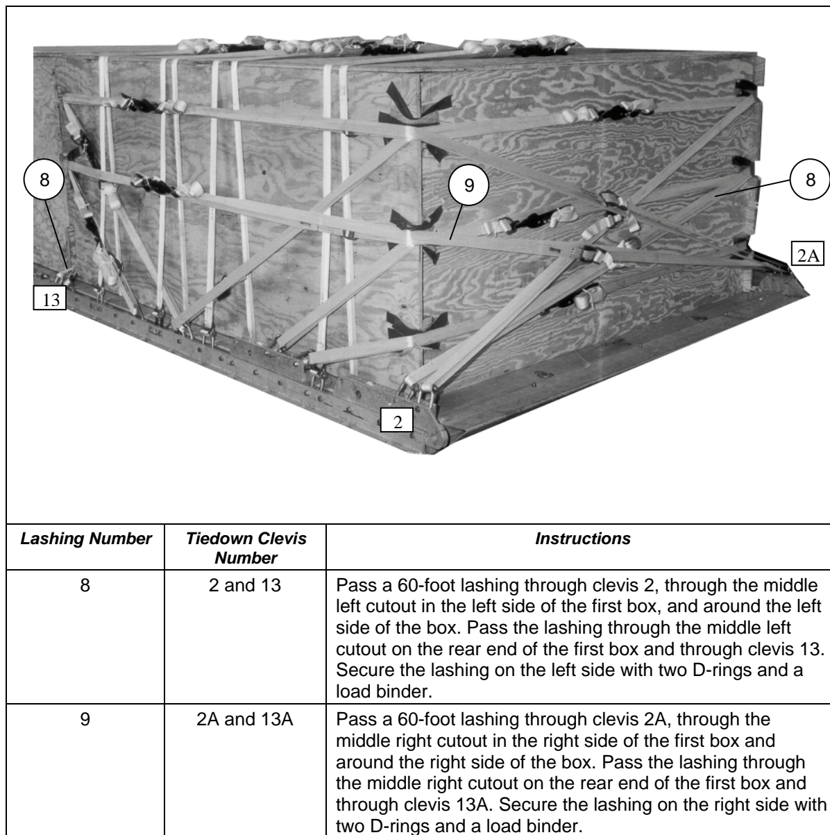
Figure 6-11. Lashings 8 and 9 Installed
