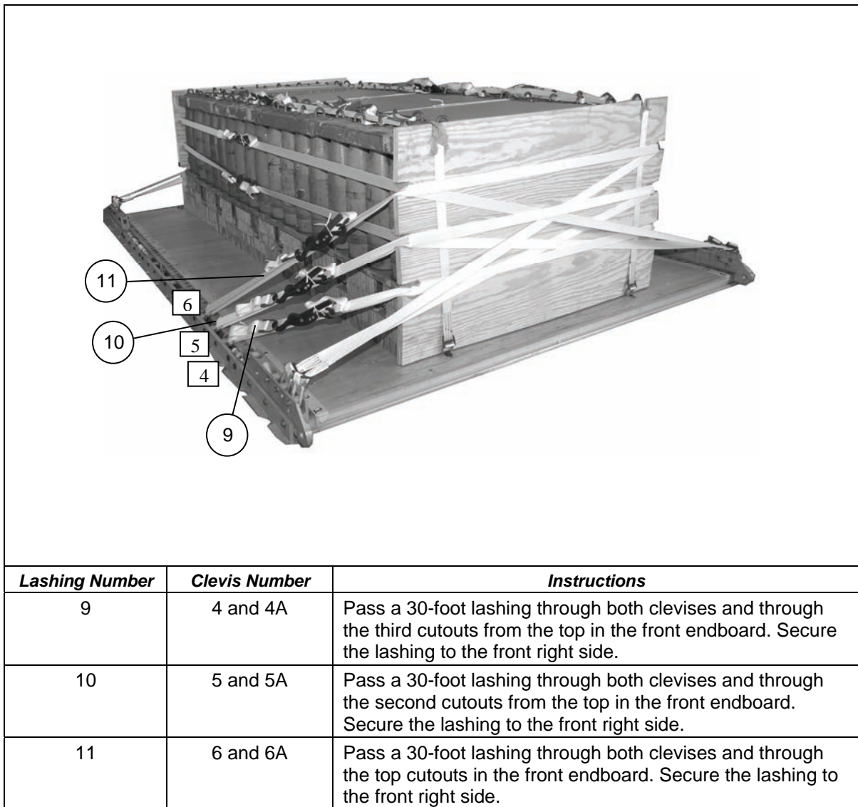
Figure 8-22. Ammunition Stack and Endboards Lashed (Continued)
