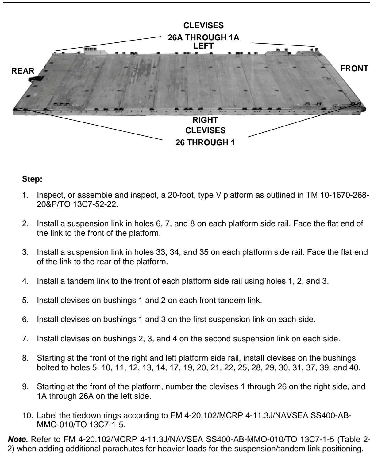
Figure 6-1. Platform Prepared
