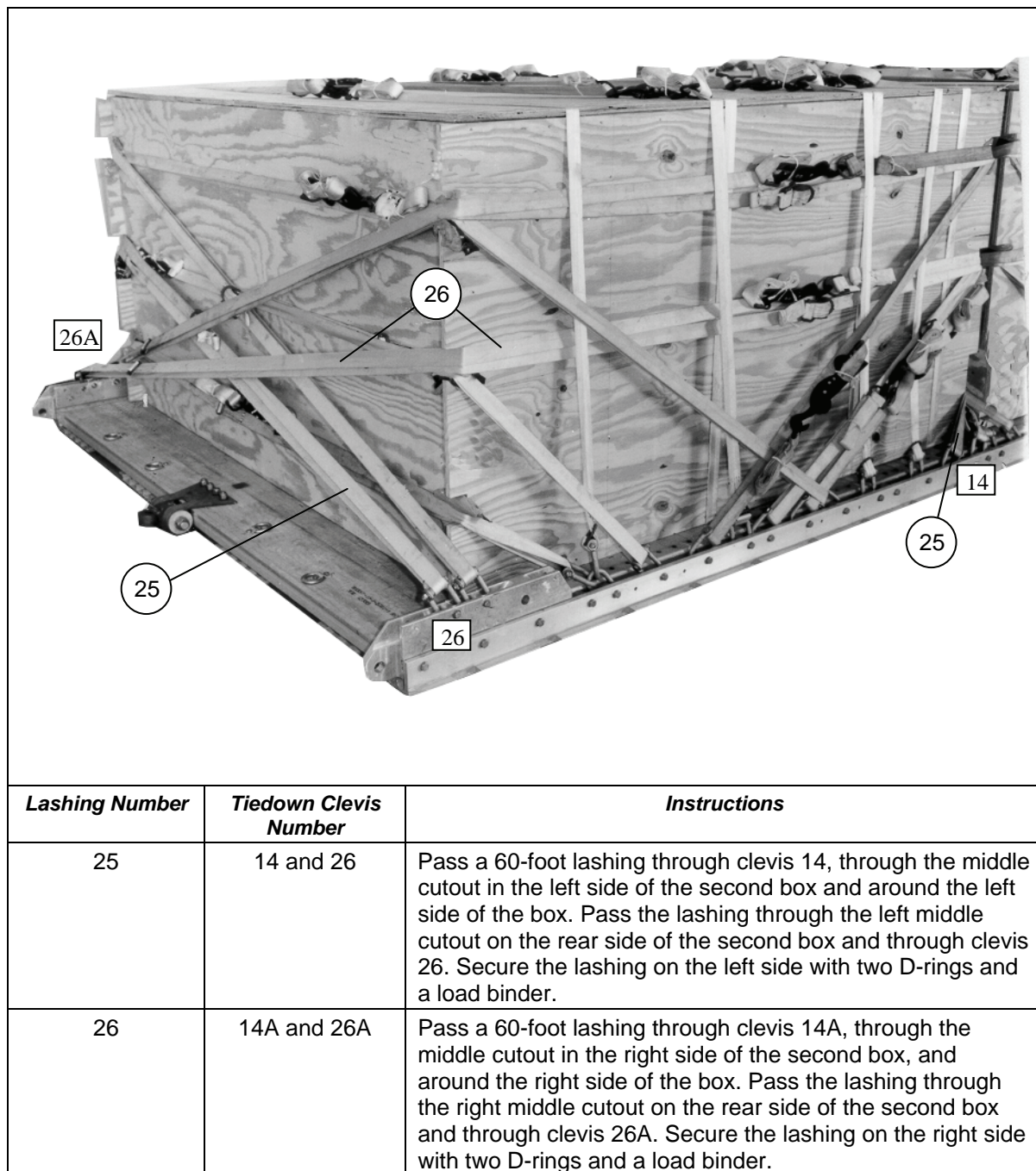
Figure 5-57. Lashings 25 and 26 Installed
