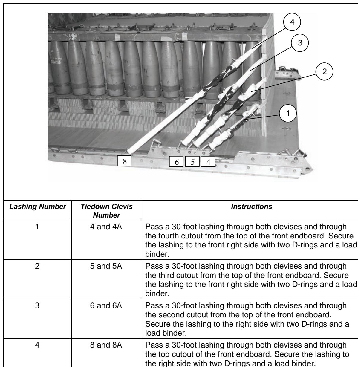
Figure 8-46. First Ammunition Stack Lashed Using the First and Second Endboards
