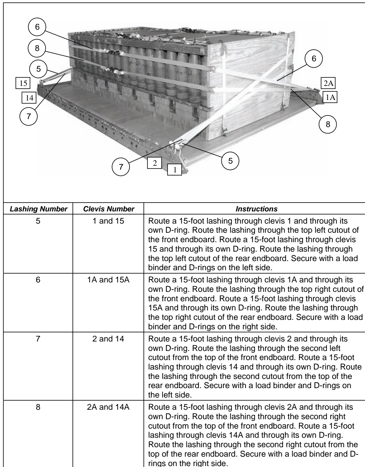
Figure 8-22. Ammunition Stack and Endboards Lashed (Continued)
