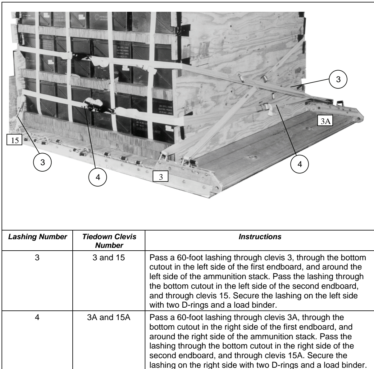
Figure 5-31. First Ammunition Stack and Endboards Lashed to Platform (Continued)
