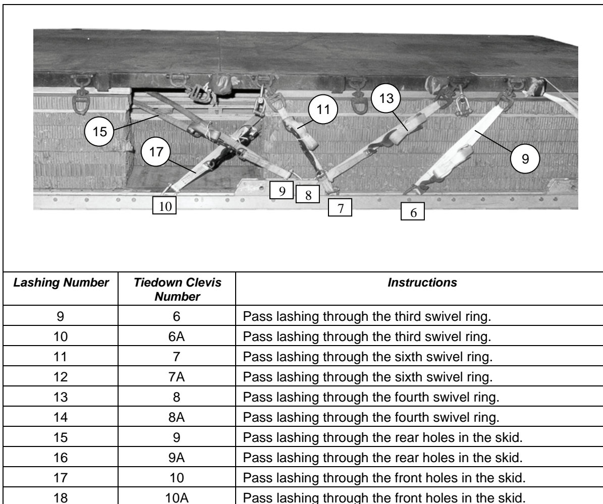
Figure 7-29. Pallet Lashed to Platform (Continued)
