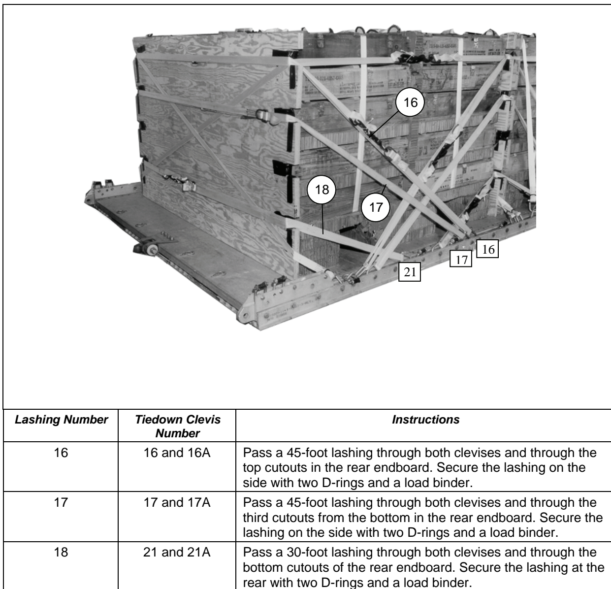
Figure 5-8. Lashings Installed for Second Stack (Continued)
