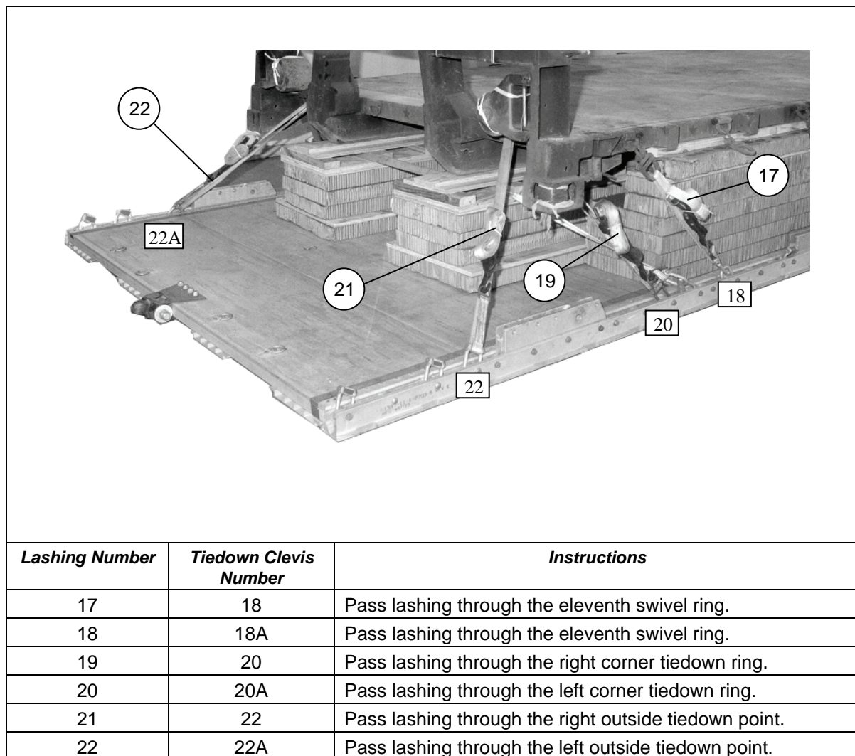
Figure 7-8. Pallet Lashed to Platform (Continued)
