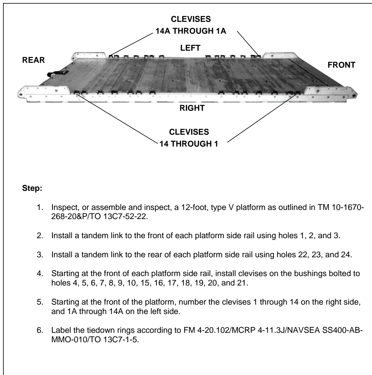
Figure 3-1. Platform Prepared
