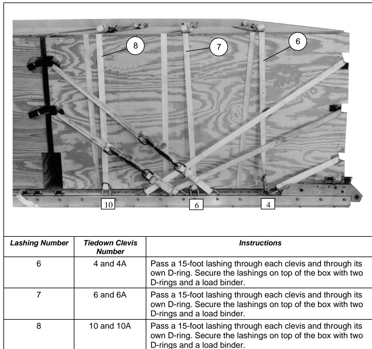
Figure 5-49. Lashings 6 Through 8 Installed
