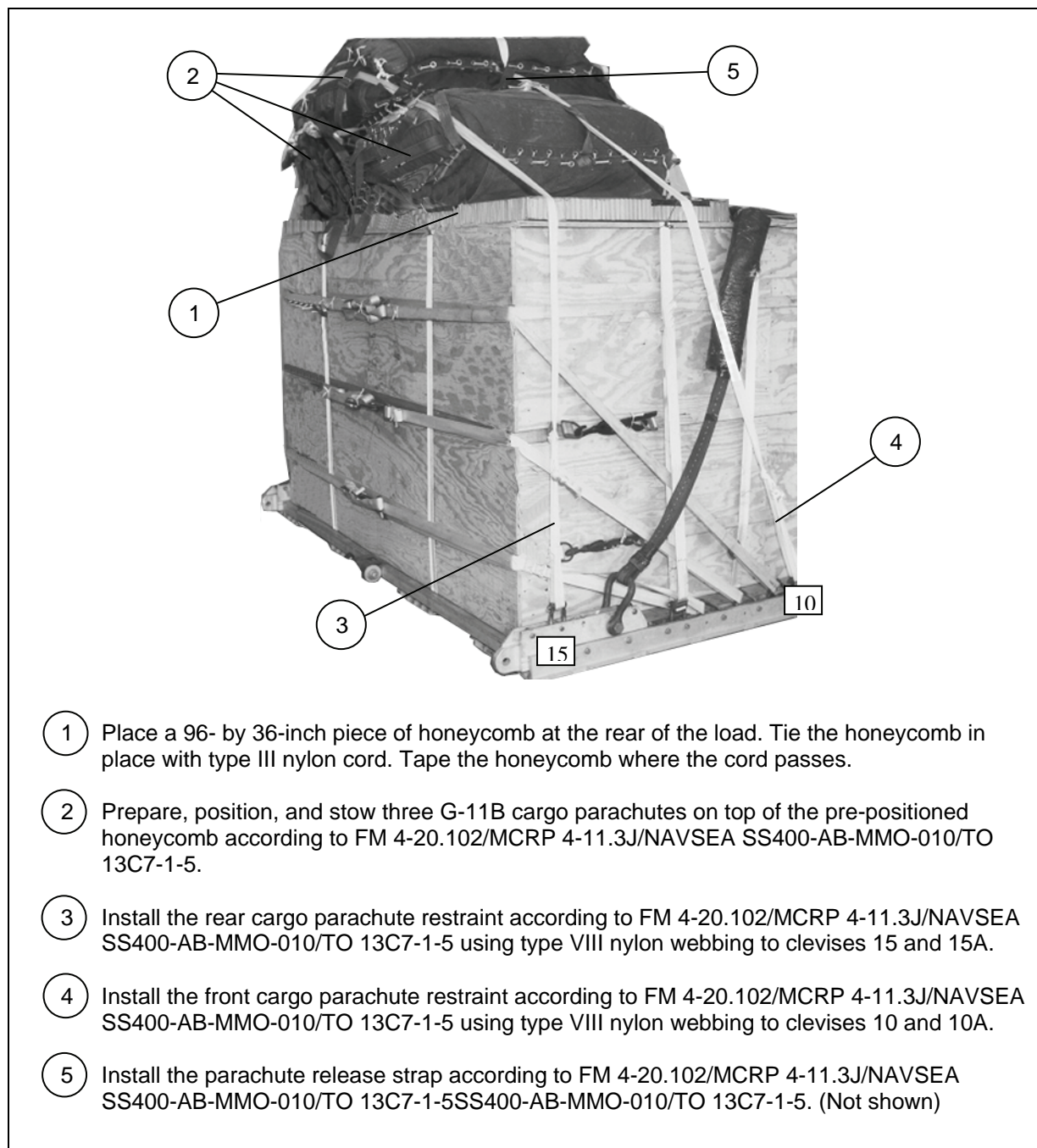
Figure 4-12. Cargo Parachutes Prepared and Stowed
