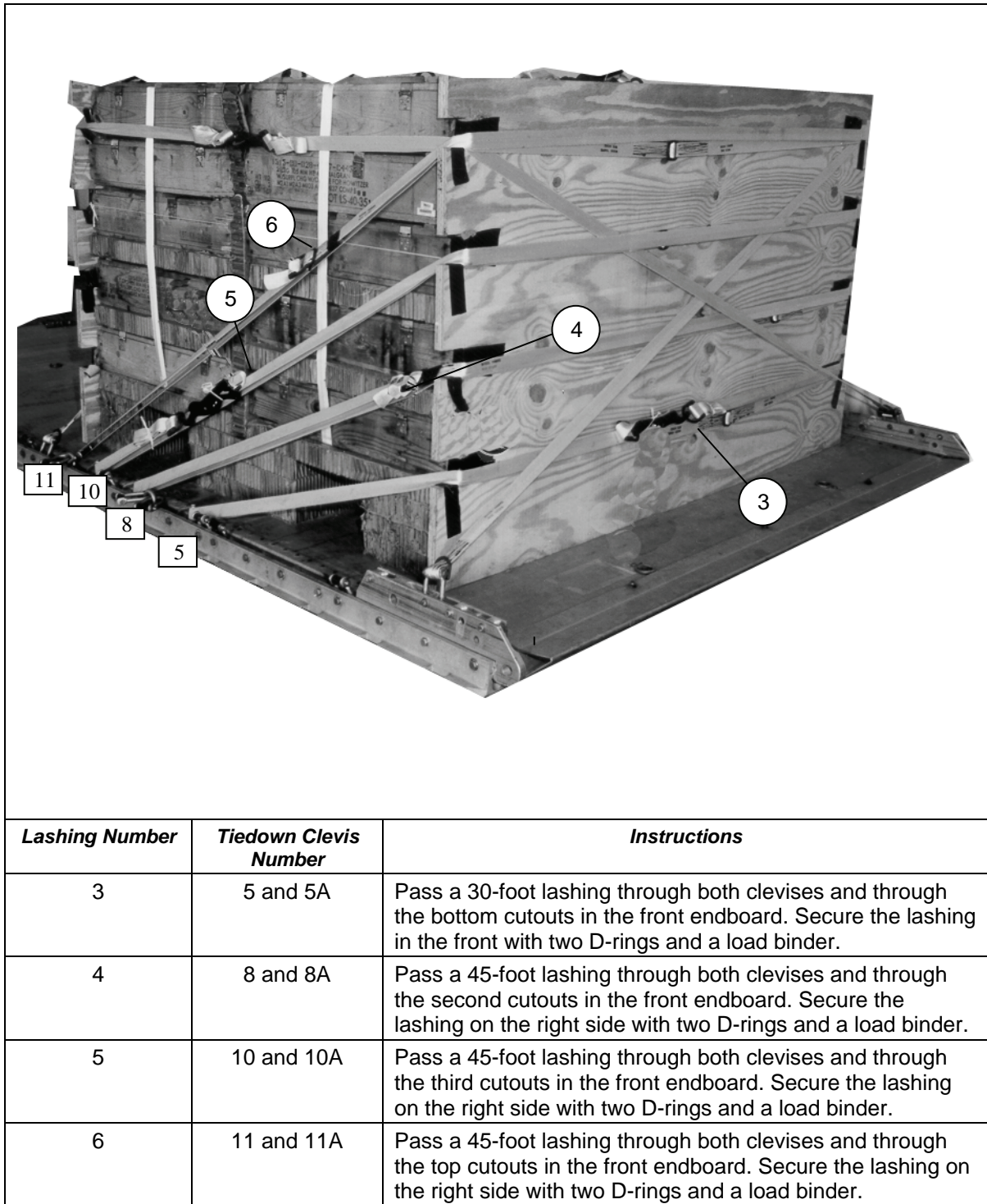
Figure 5-5. Lashings Installed for First Stack (Continued)
