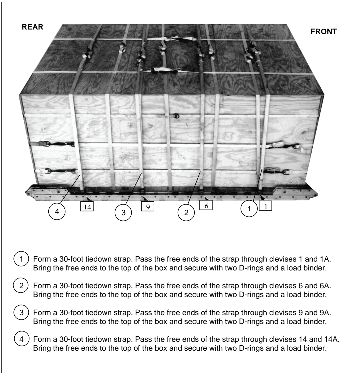
Figure 4-10. Lashings Installed
