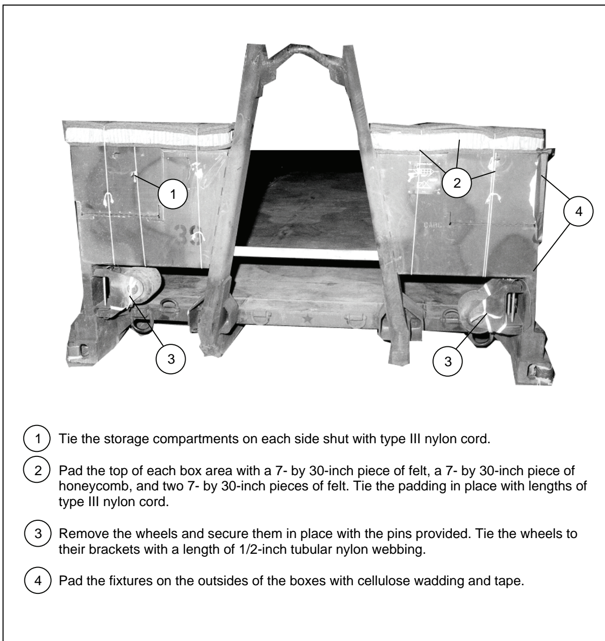
Figure 7-27. Pallet Prepared
