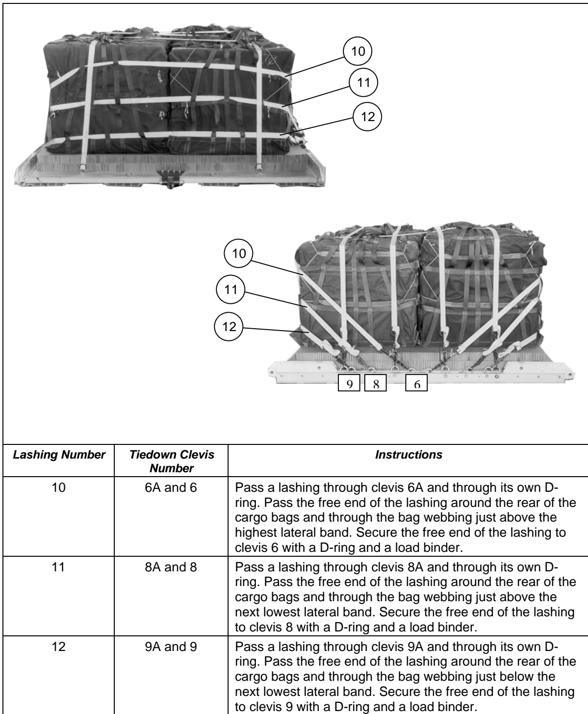
Figure 2-19. Lashings 10 Through 12 Installed
