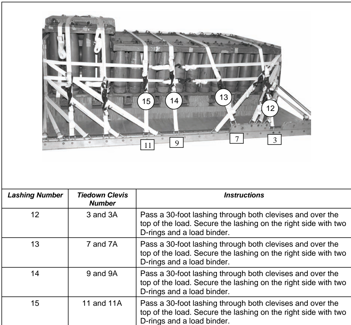
Figure 8-46. First Ammunition Stack Lashed Using the First and Second Endboards (Continued)
