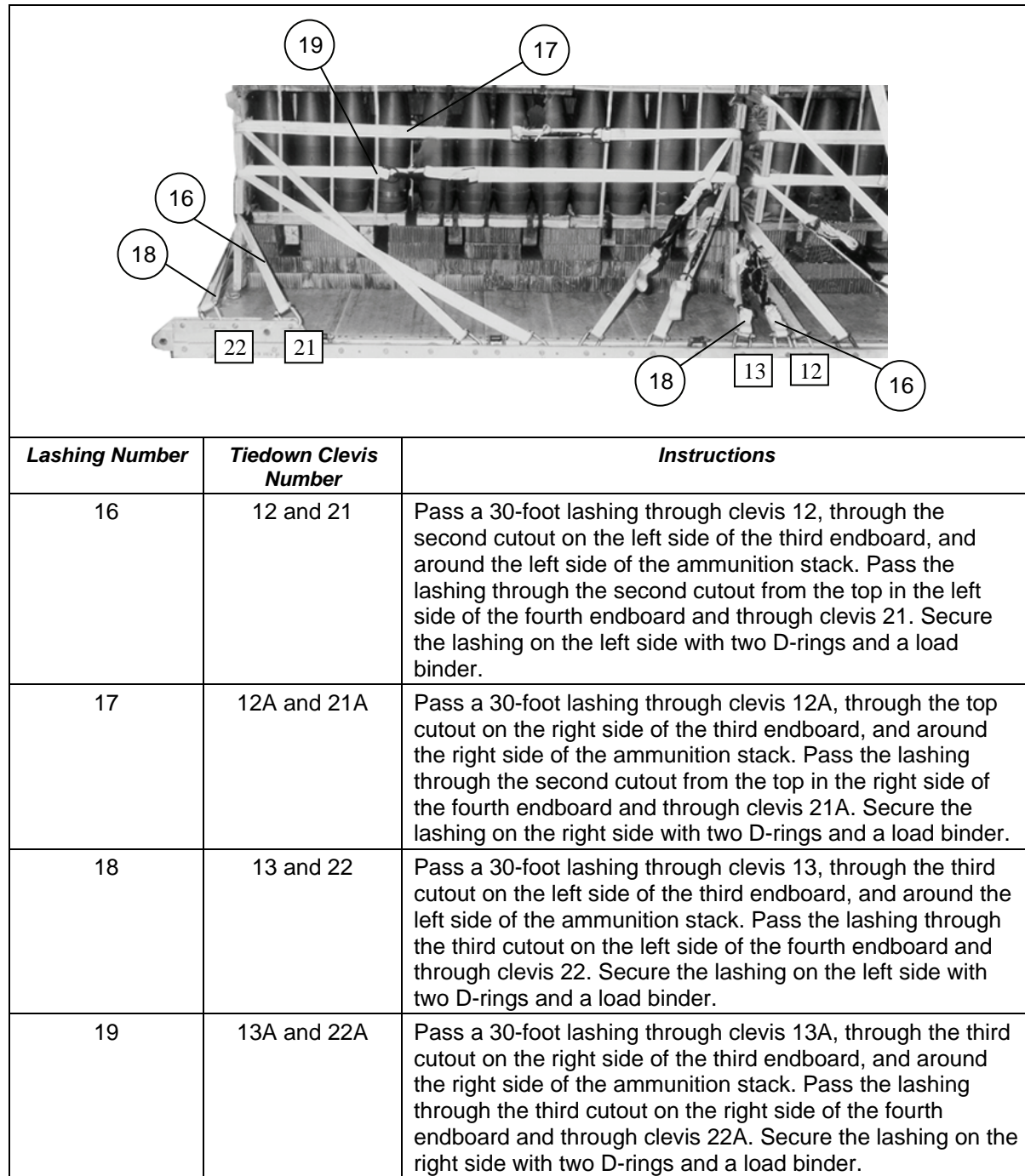
Figure 5-20. Lashings Installed for Second Stack (Continued)
