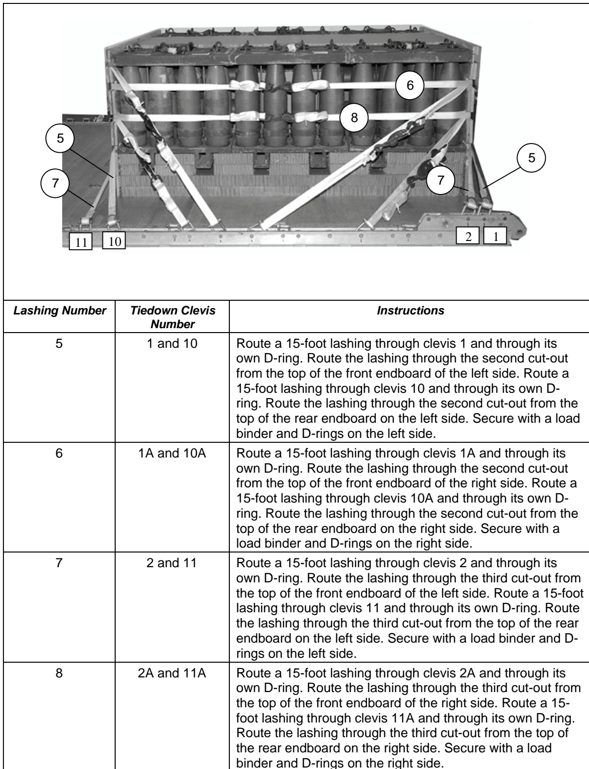
Figure 8-33. First Ammunition Stack Lashed Using the First and Second Endboards (Continued)
