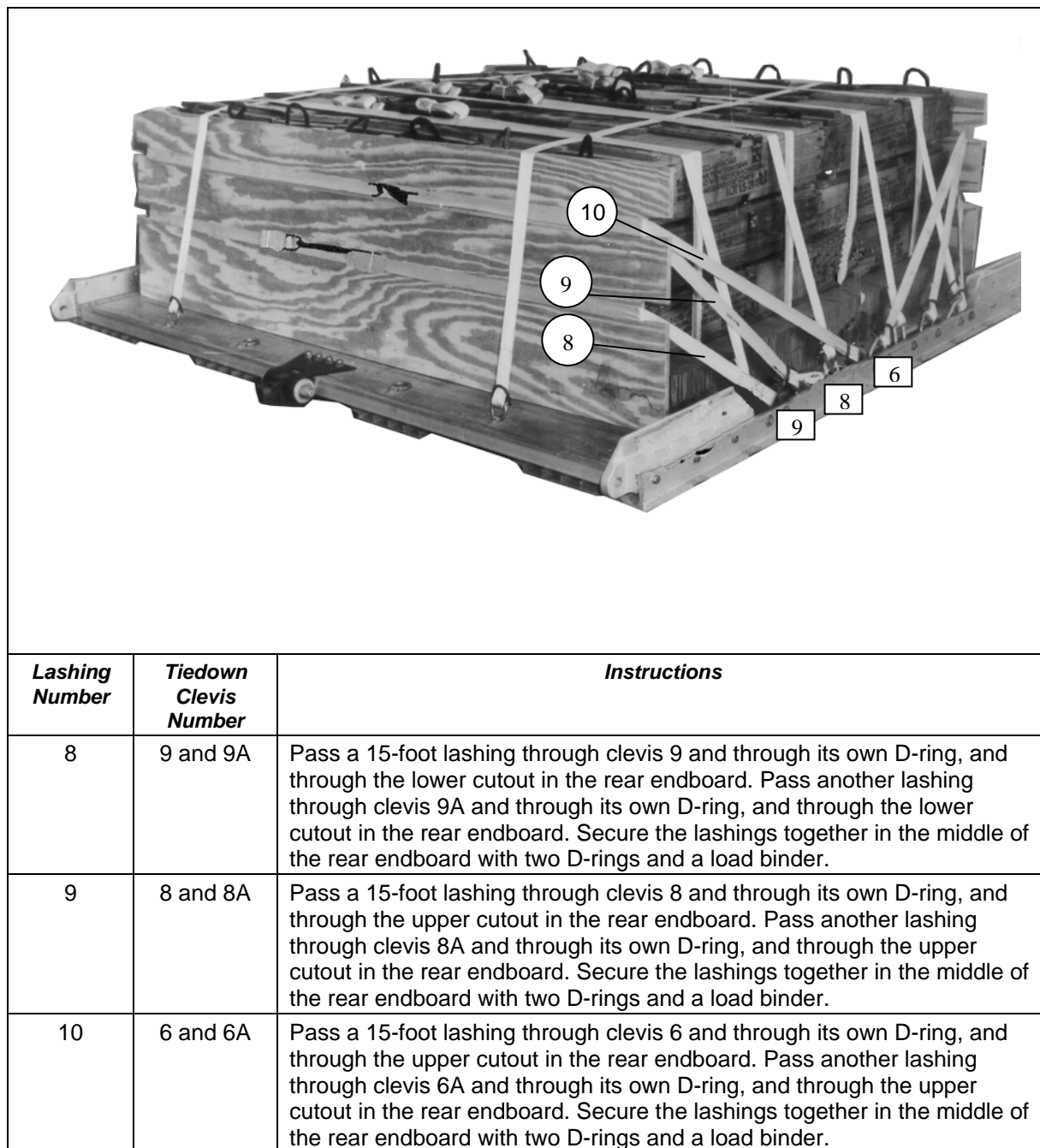
Figure 2-7. Lashings 8 Through 10 Installed
