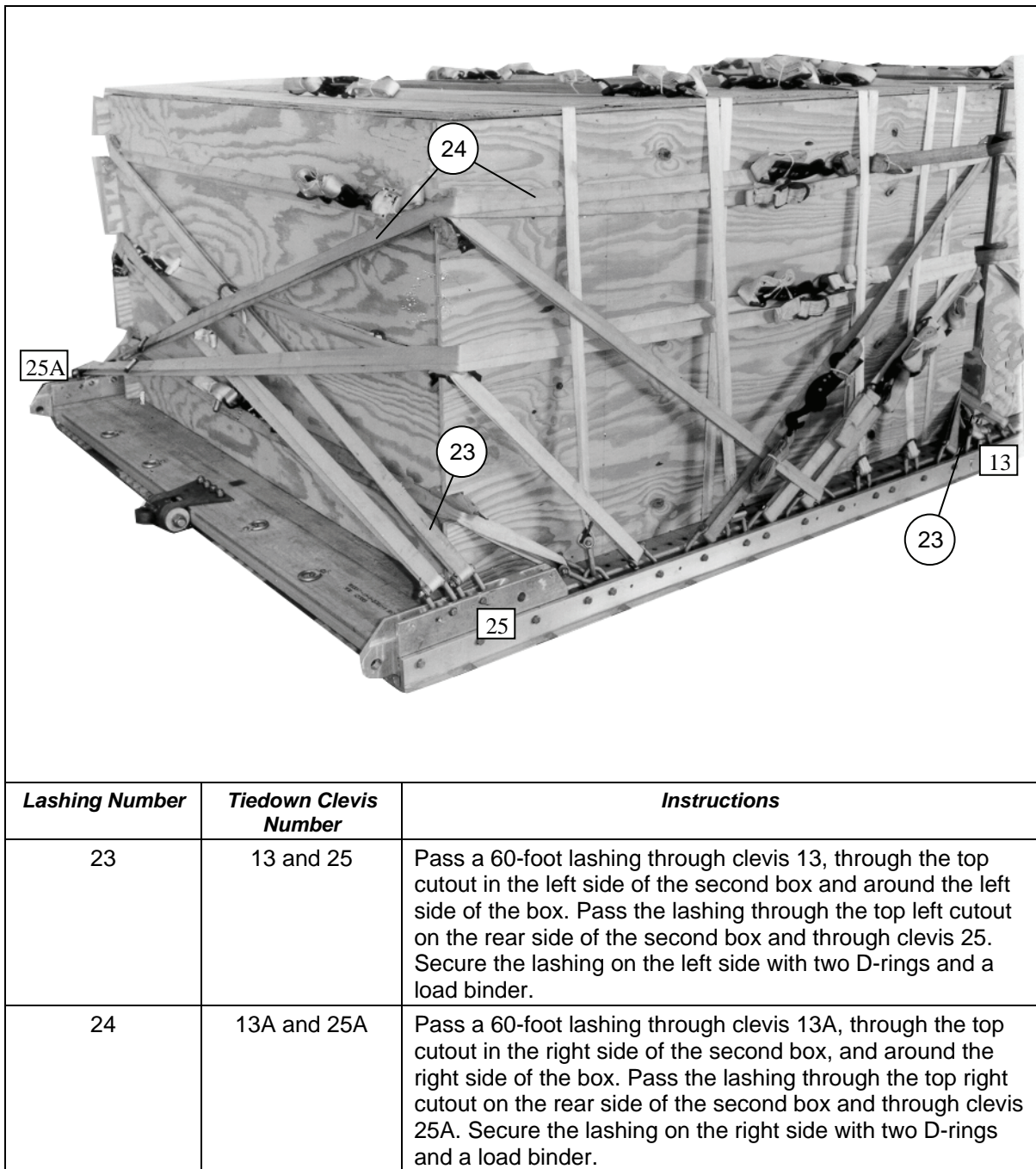
Figure 5-56. Lashings 23 and 24 Installed
