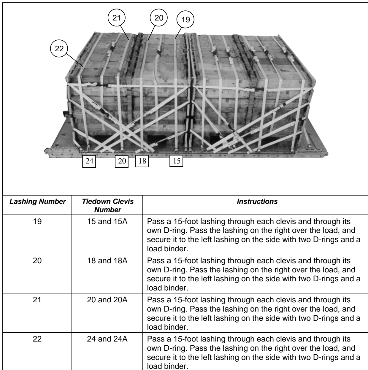
Figure 5-8. Lashings Installed for Second Stack (Continued)
