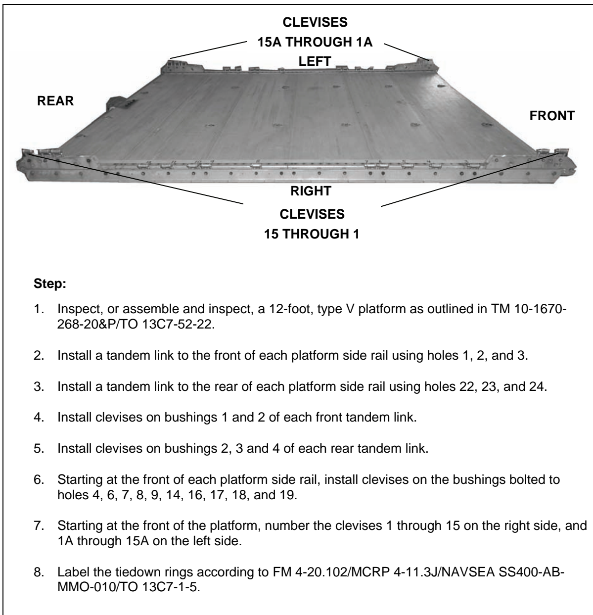
Figure 8-14. Platform Prepared
