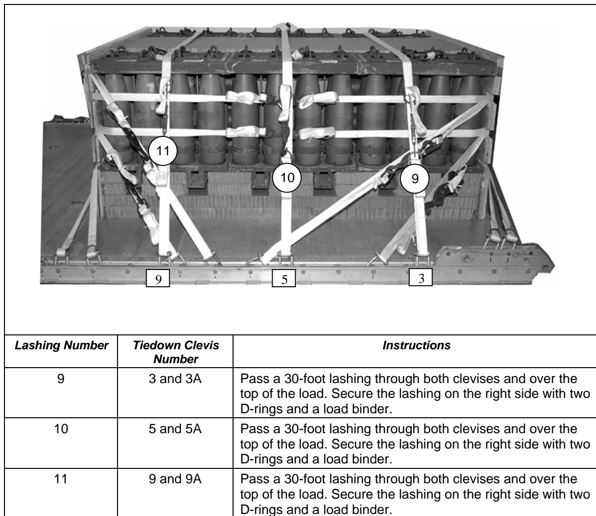
Figure 8-33. First Ammunition Stack Lashed Using the First and Second Endboards (Continued)
