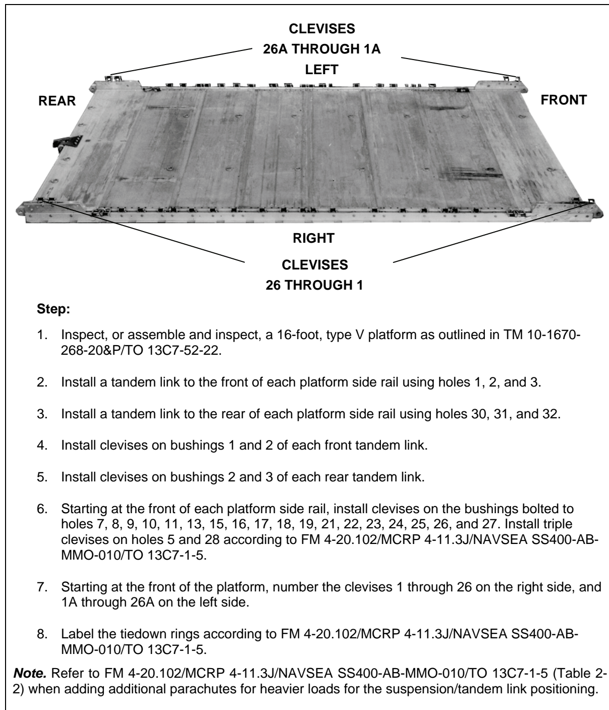
Figure 5-41. Platform Prepared
