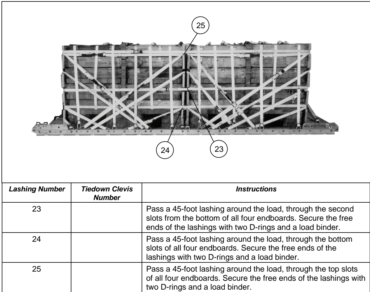
Figure 5-8. Lashings Installed for Second Stack (Continued)
