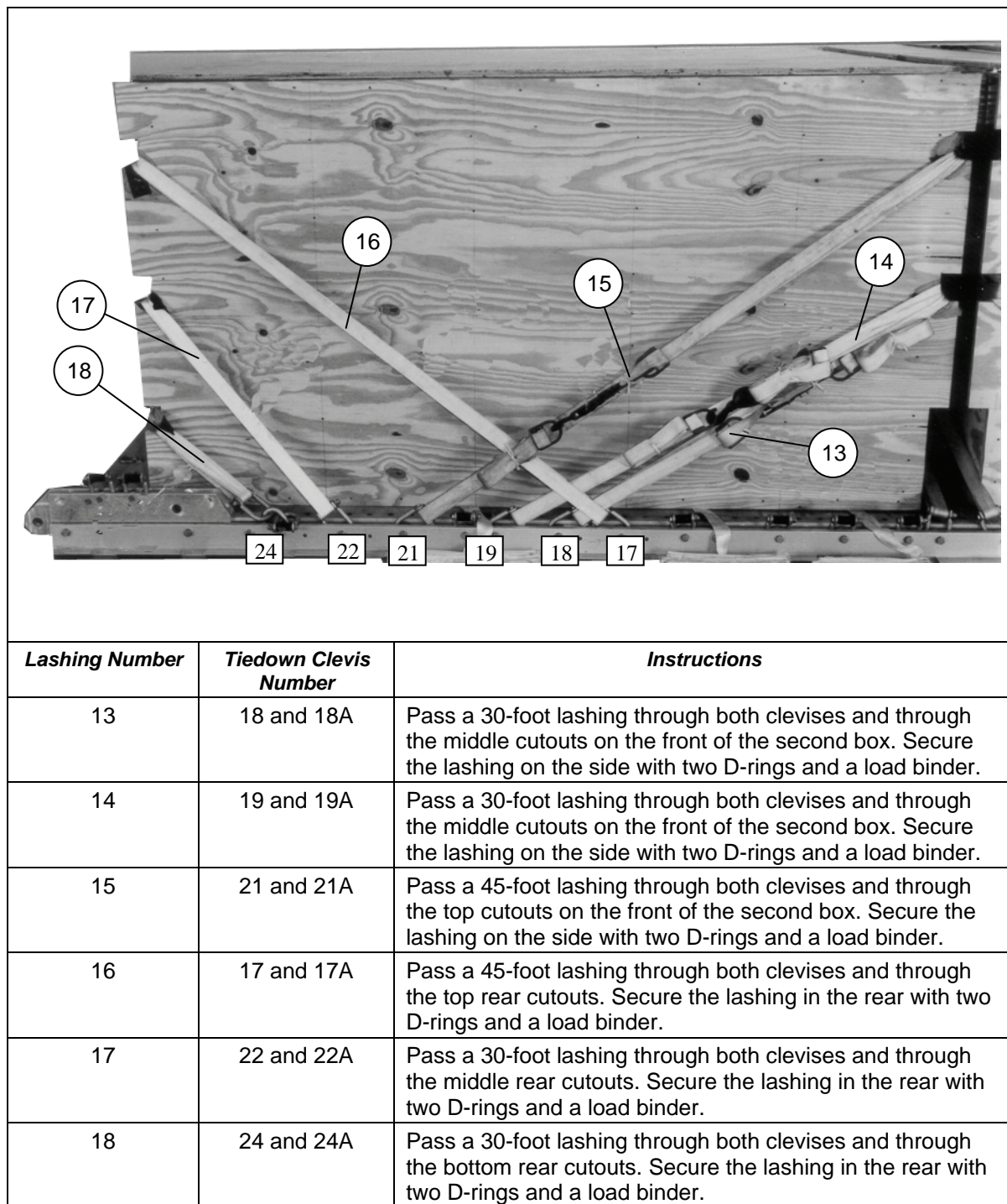
Figure 5-53. Lashings 13 Through 18 Installed
