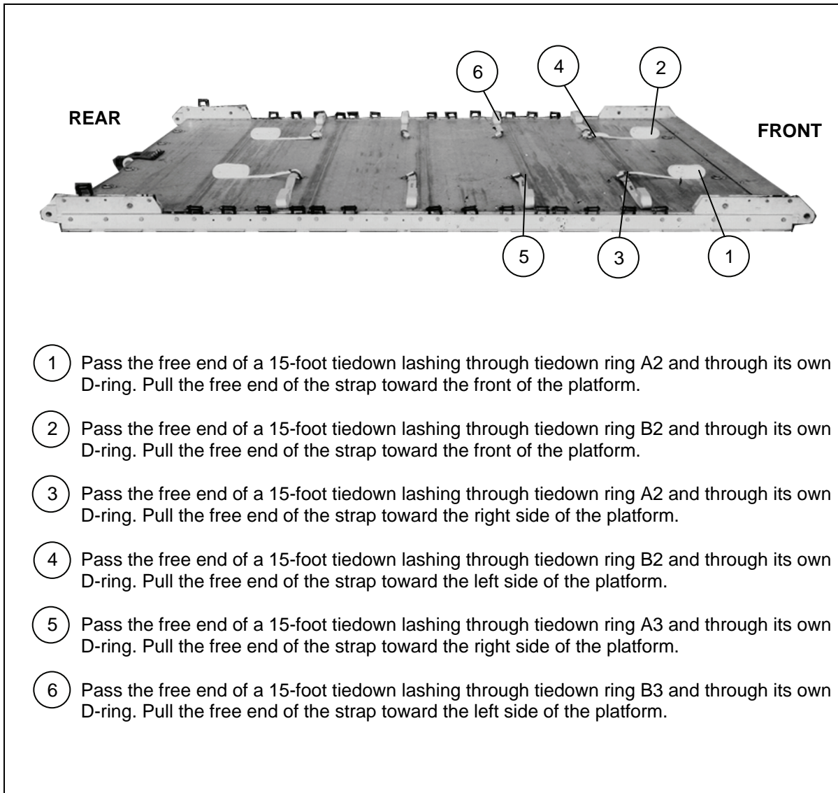
Figure 4-2. Lashings Positioned
