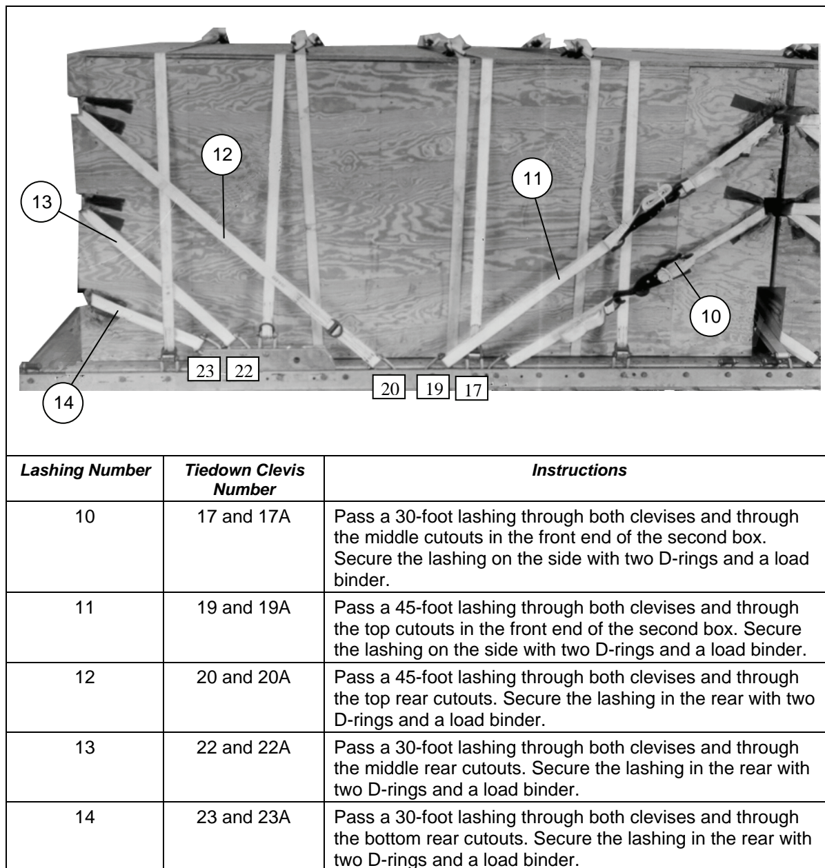
Figure 6-13. Lashings 10 Through 14 Installed
