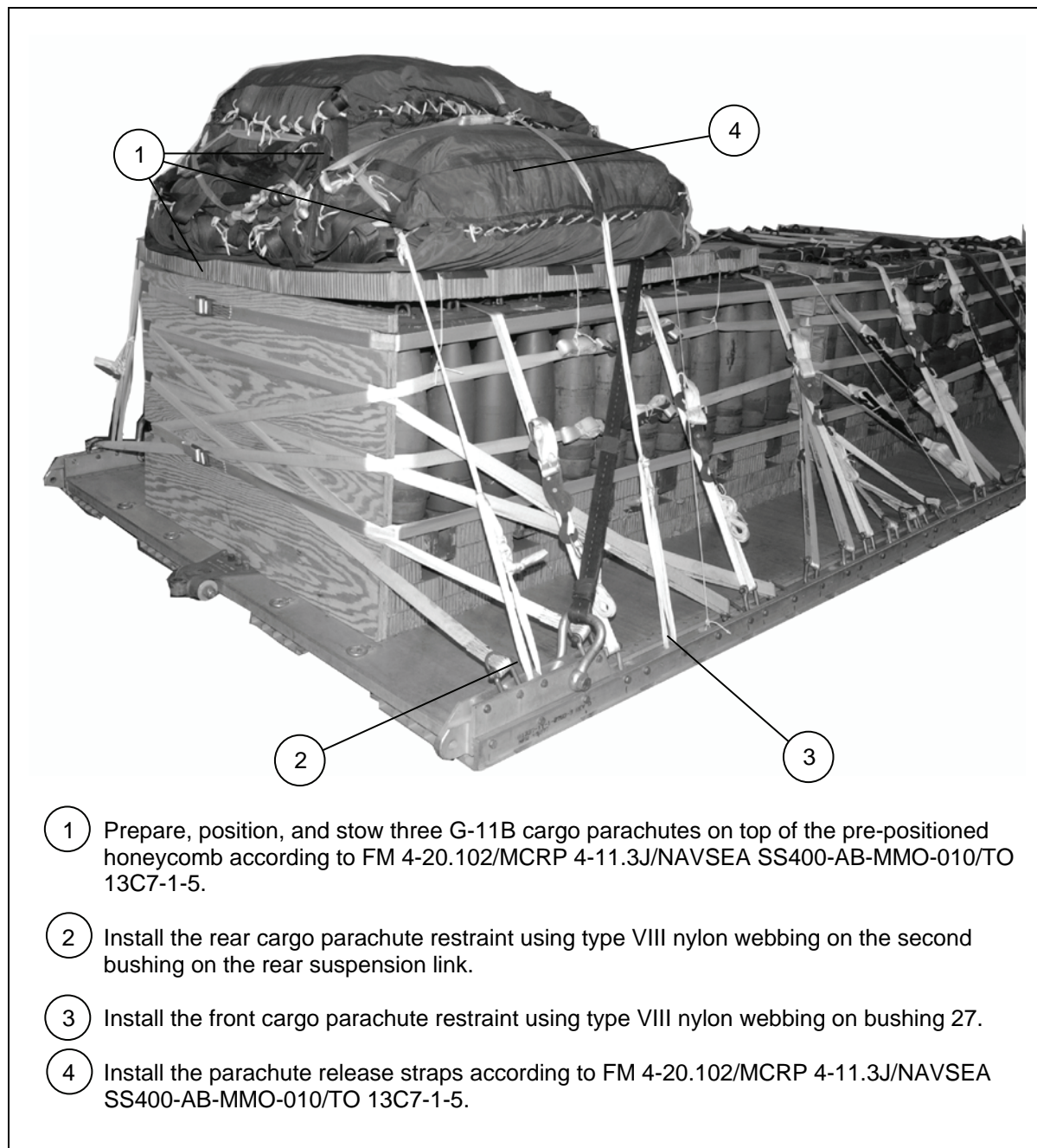
Figure 8-38. Cargo Parachutes Prepared and Stowed
