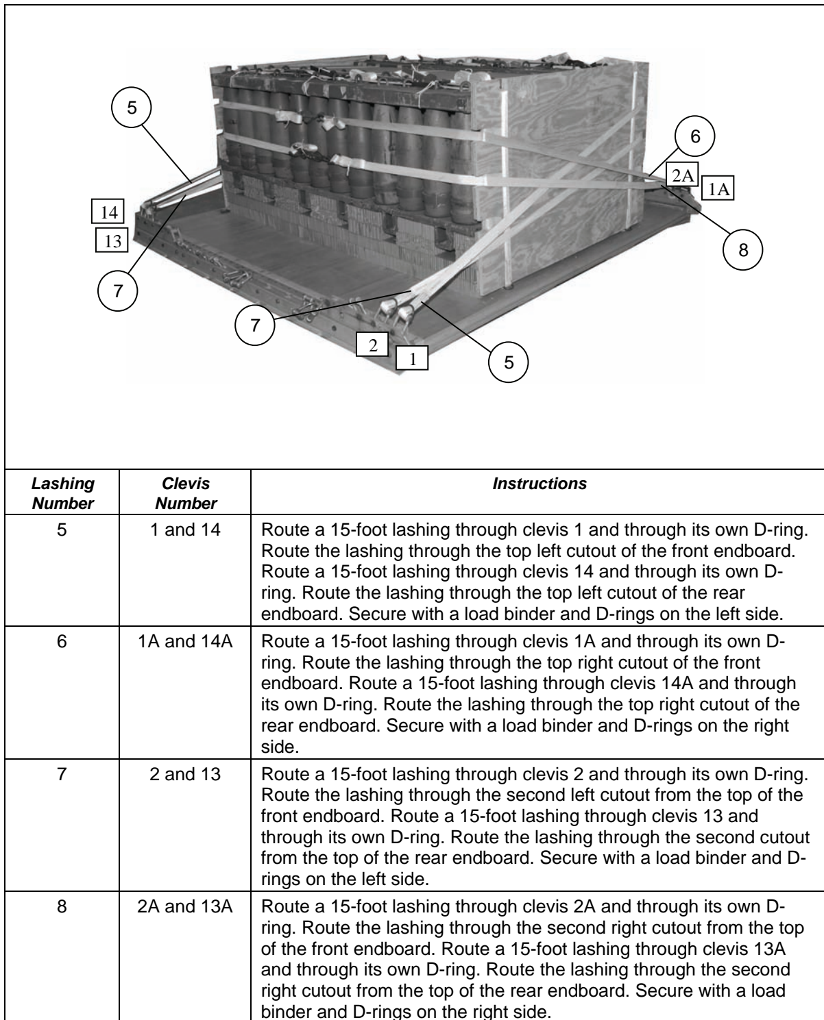
Figure 8-8. Ammunition Stack and Endboards Lashed (Continued)
