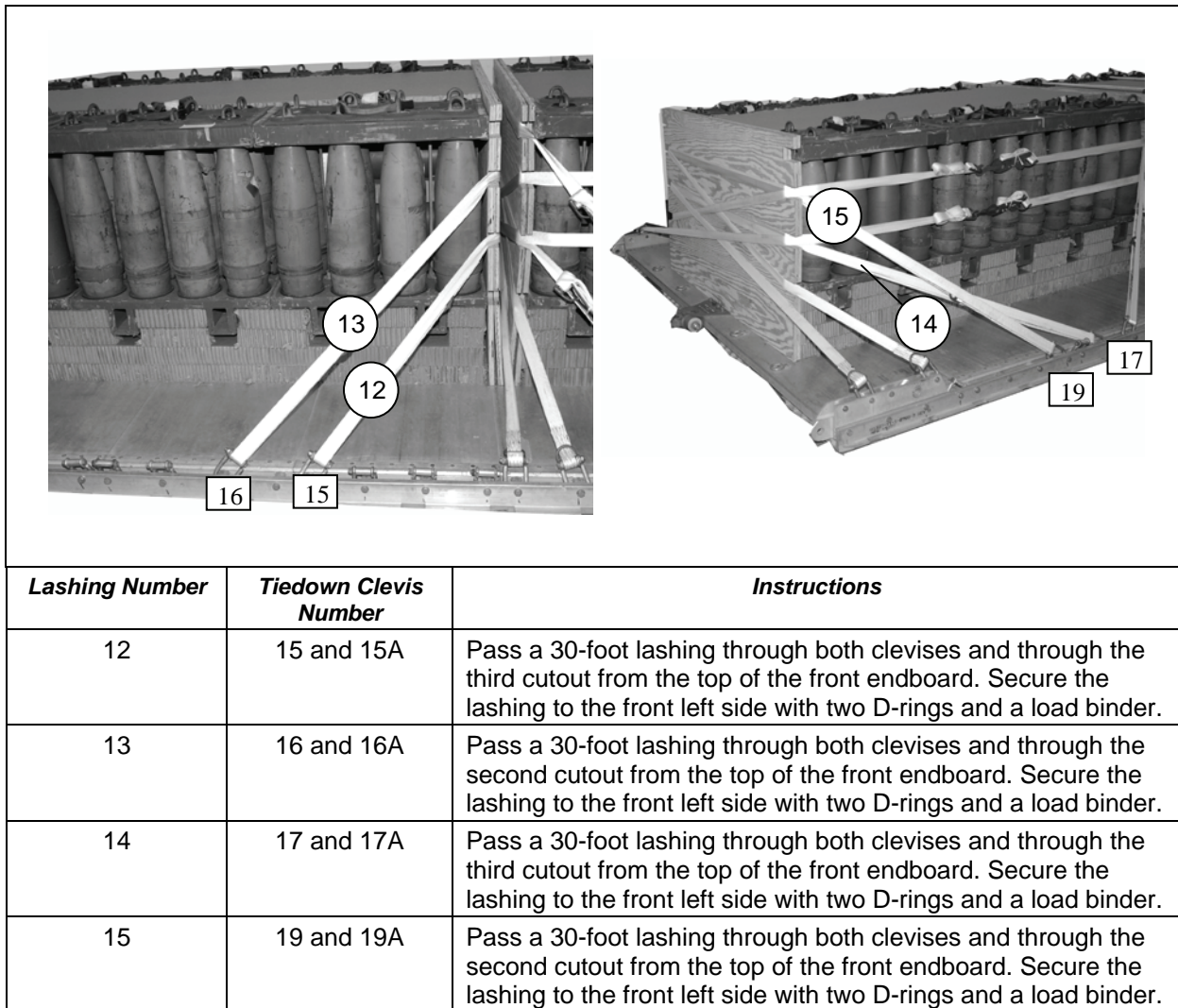
Figure 8-35. Second Ammunition Stack Lashed Using the Third and Fourth Endboards
