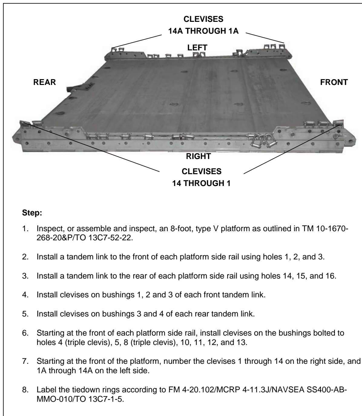
Figure 8-1. Platform Prepared
