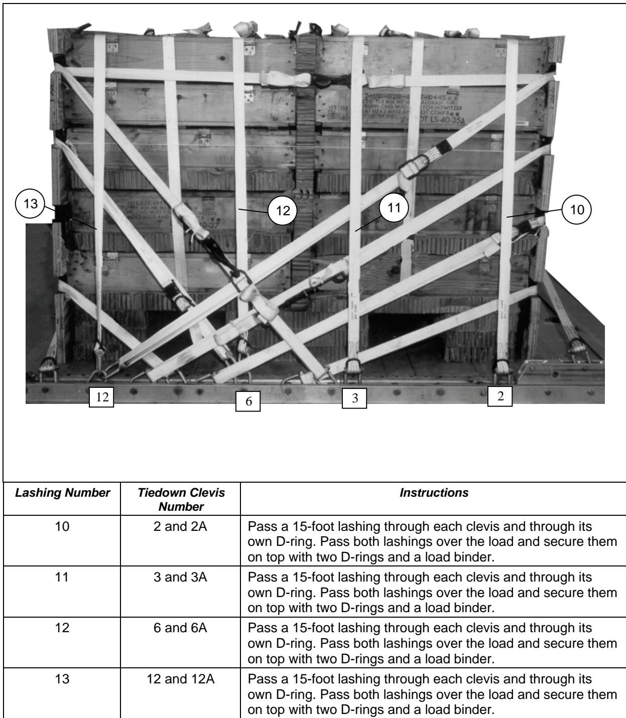
Figure 5-5. Lashings Installed for First Stack (Continued)
