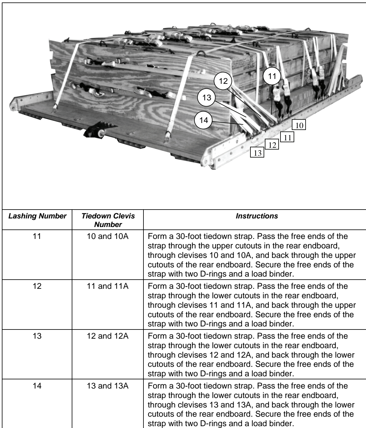
Figure 3-7. Lashings 11 Through 14 Installed
