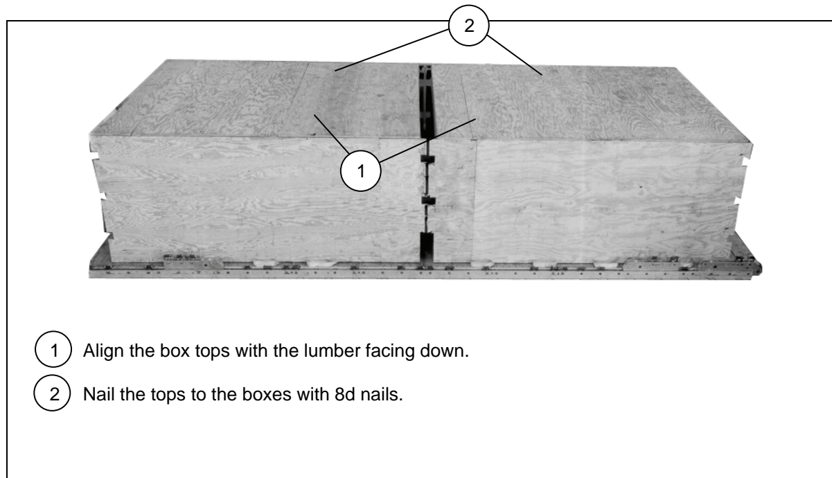
Figure 6-7. Boxes Closed
