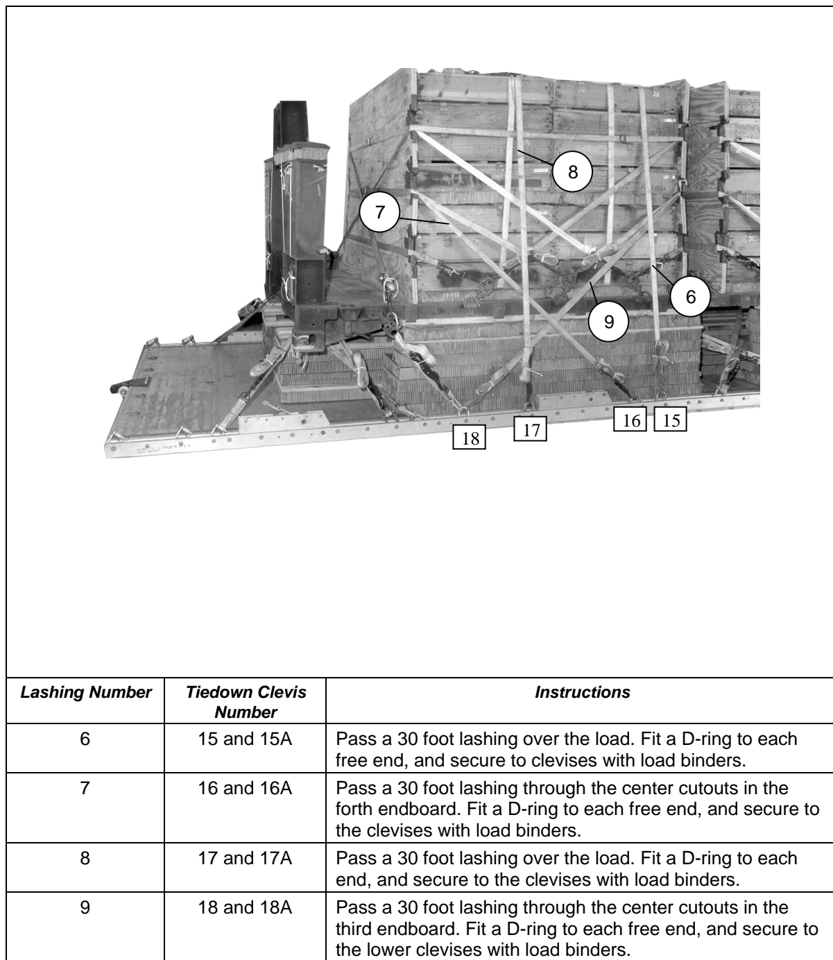
Figure 7-14. Load Lashed to Platform (Continued)
