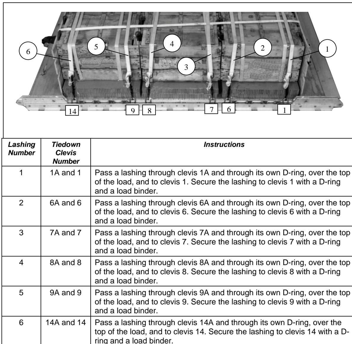
Figure 3-5. Lashings 1 Through 6 Installed
