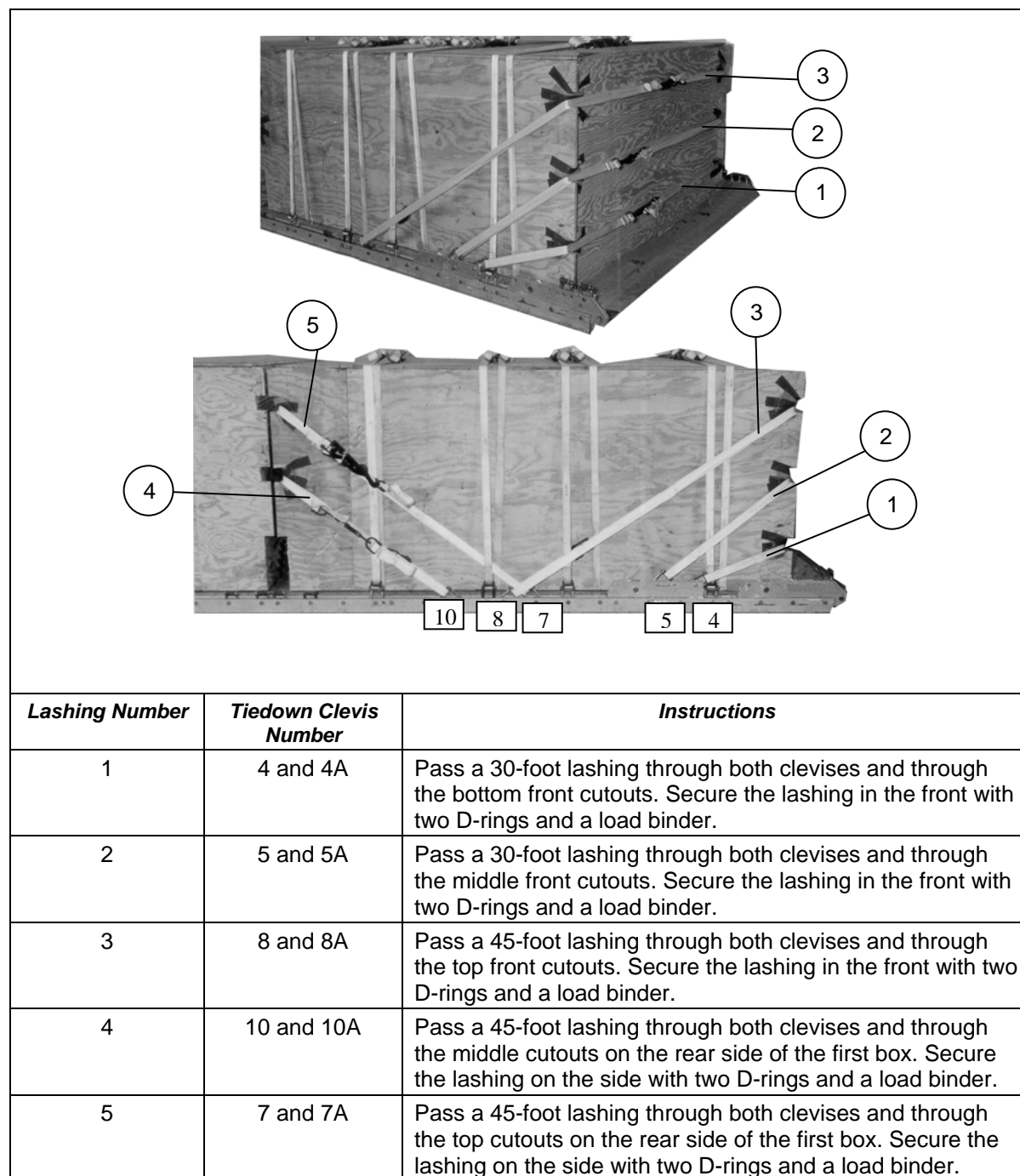
Figure 6-9. Lashings 1 Through 5 Installed
