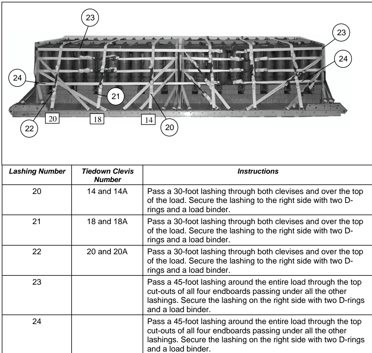
Figure 8-35. Second Ammunition Stack Lashed Using the Third and Fourth Endboards (Continued)
