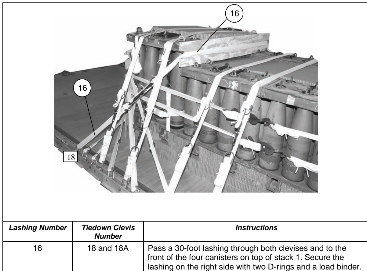
Figure 8-46. First Ammunition Stack Lashed Using the First and Second Endboards (Continued)
