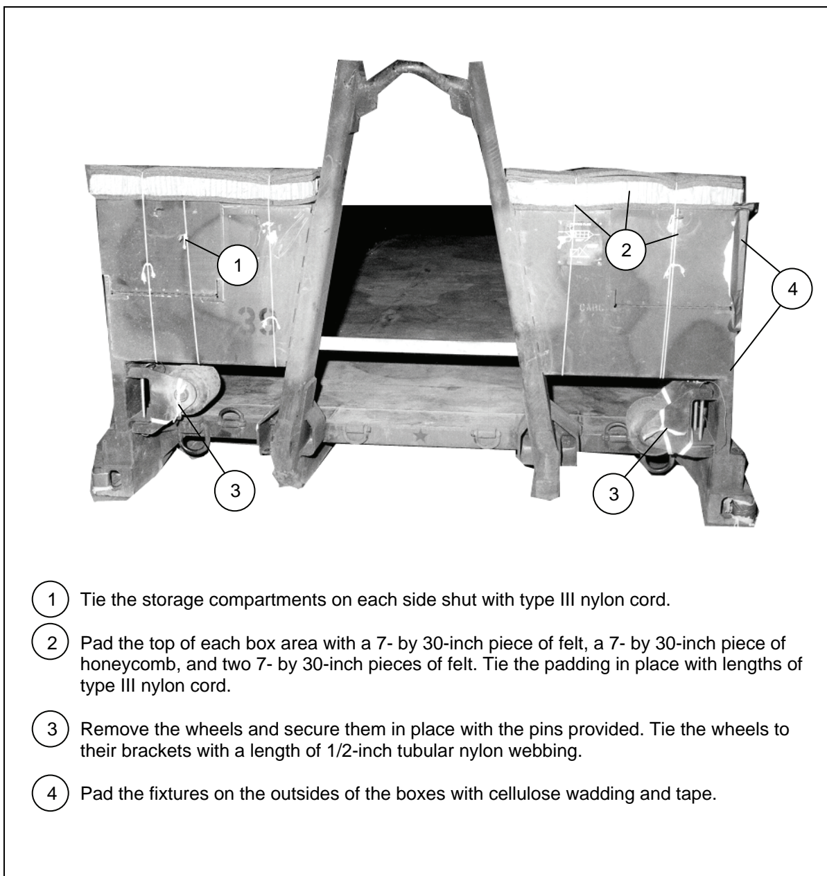
Figure 7-6. Pallet Prepared
