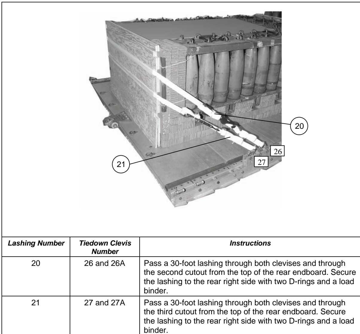
Figure 8-49. Second Ammunition Stack Lashed Using the Third and Fourth Endboards (Continued)
