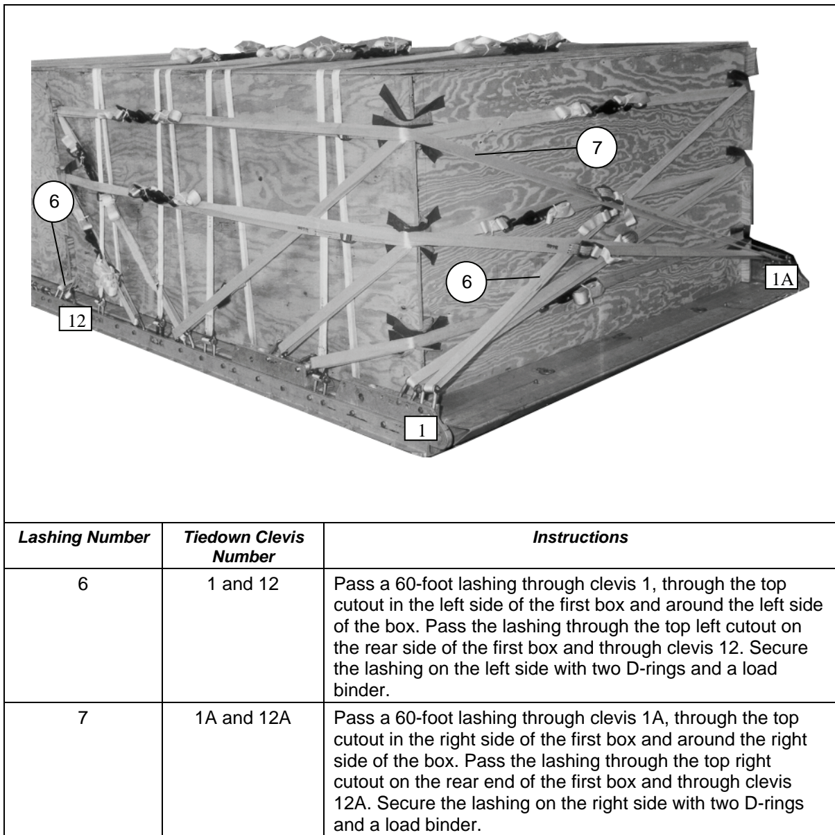
Figure 6-10. Lashings 6 and 7 Installed
