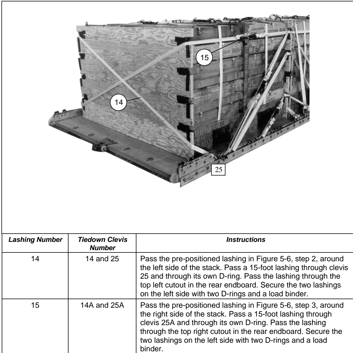
Figure 5-8. Lashings Installed for Second Stack
