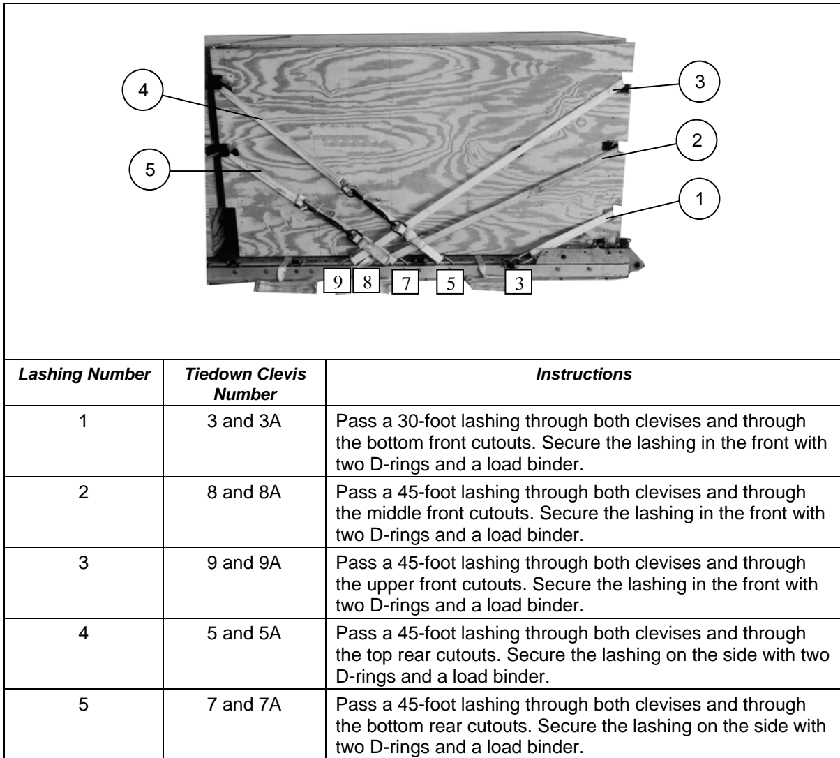
Figure 5-48. Lashings 1 Through 5 Installed
