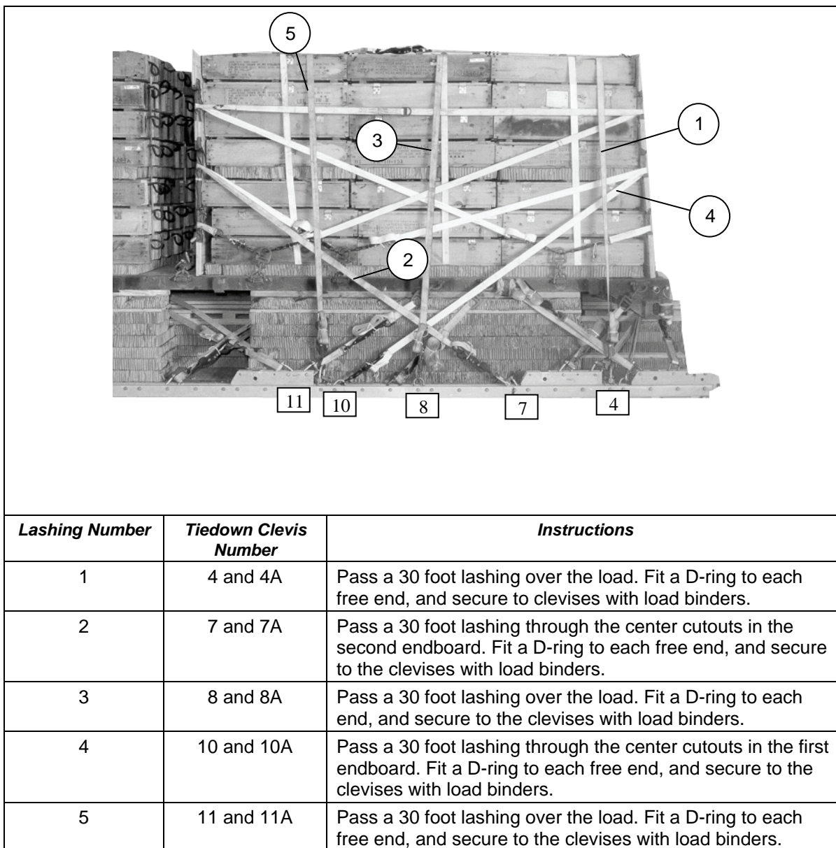
Figure 7-14. Load Lashed to Platform
