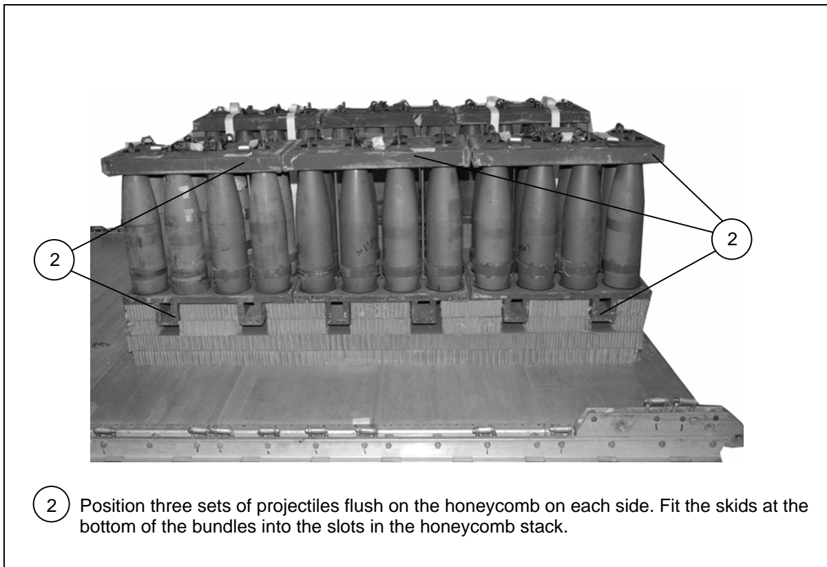
Figure 8-31. Ammunition Positioned and Secured (Continued)
