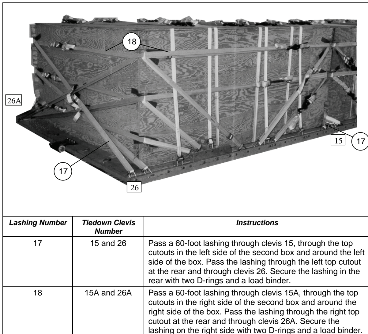
Figure 6-15. Lashings 17 and 18 Installed
