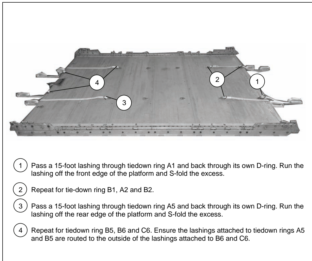
Figure 8-17. Lashings Positioned on Platform
