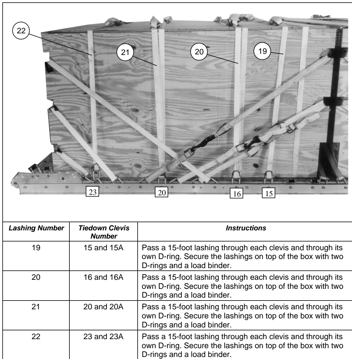
Figure 5-55. Lashings 19 Through 22 Installed
