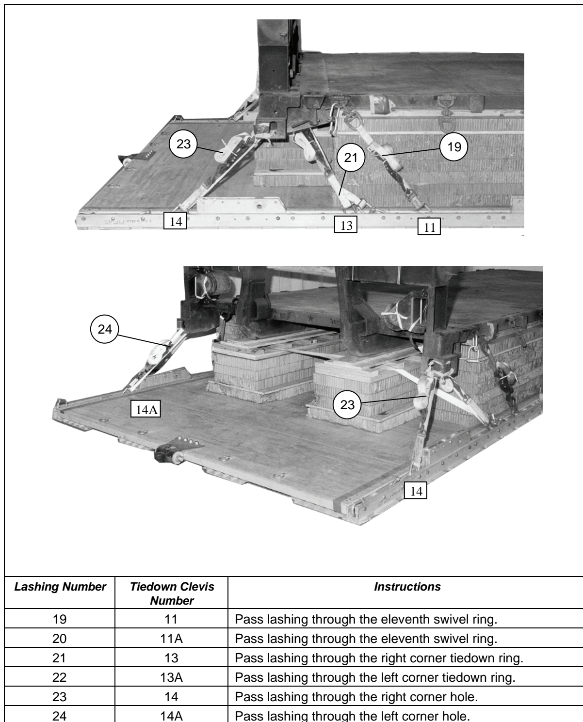
Figure 7-29. Pallet Lashed to Platform (Continued)
