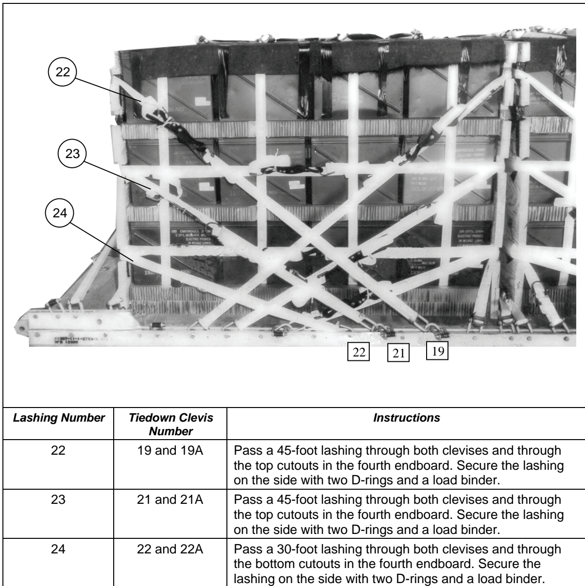
Figure 5-34. Second Ammunition Stack and Endboards Lashed to Platform (Continued)
