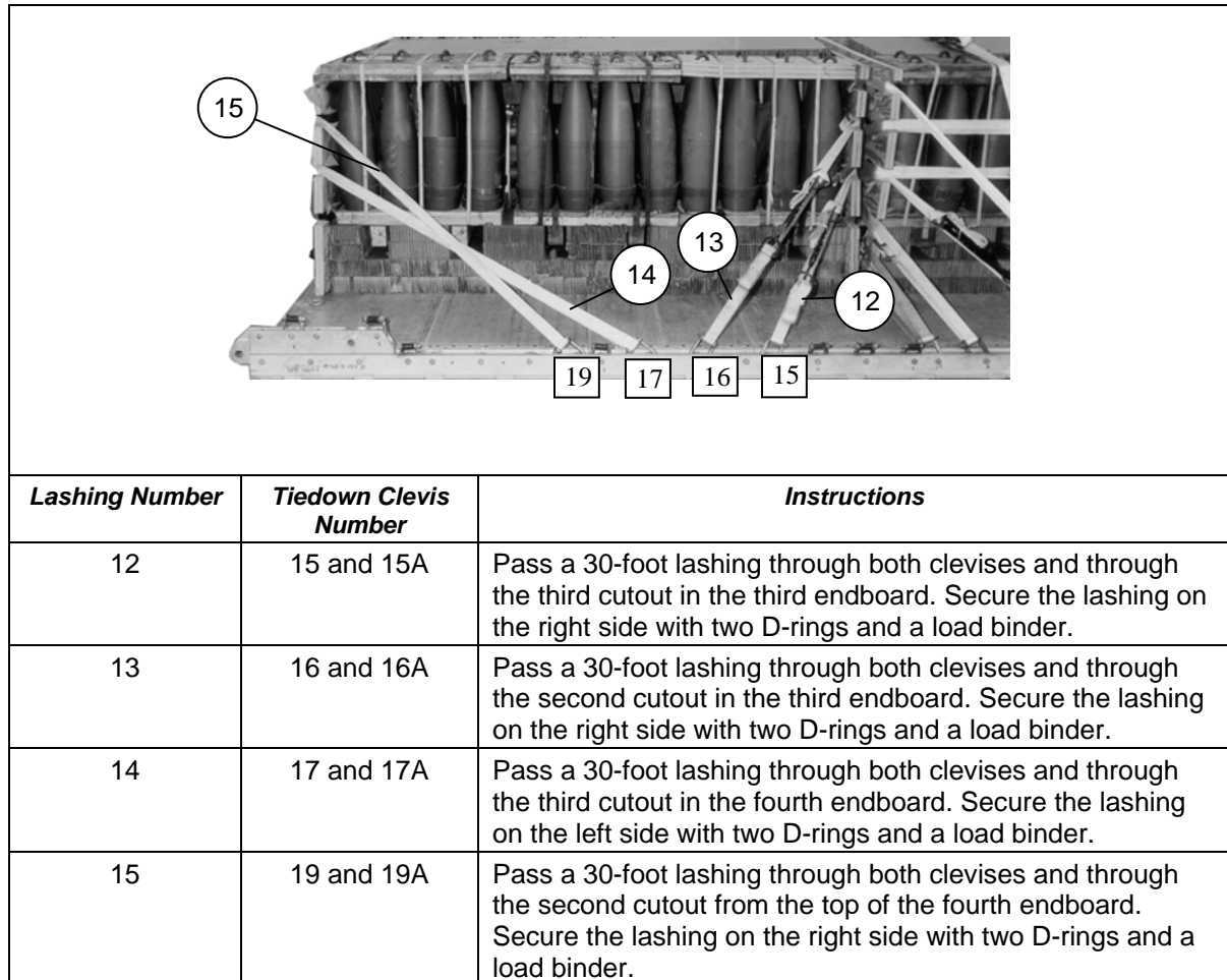
Figure 5-20. Lashings Installed for Second Stack
