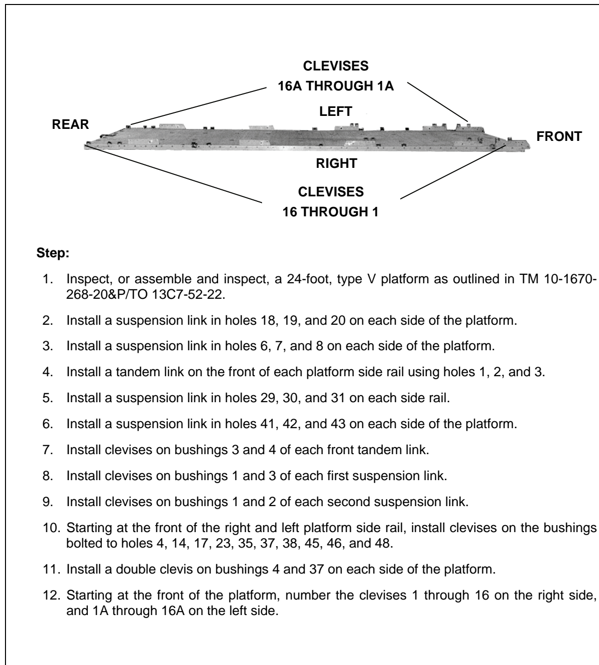
Figure 7-22. Platform Prepared
