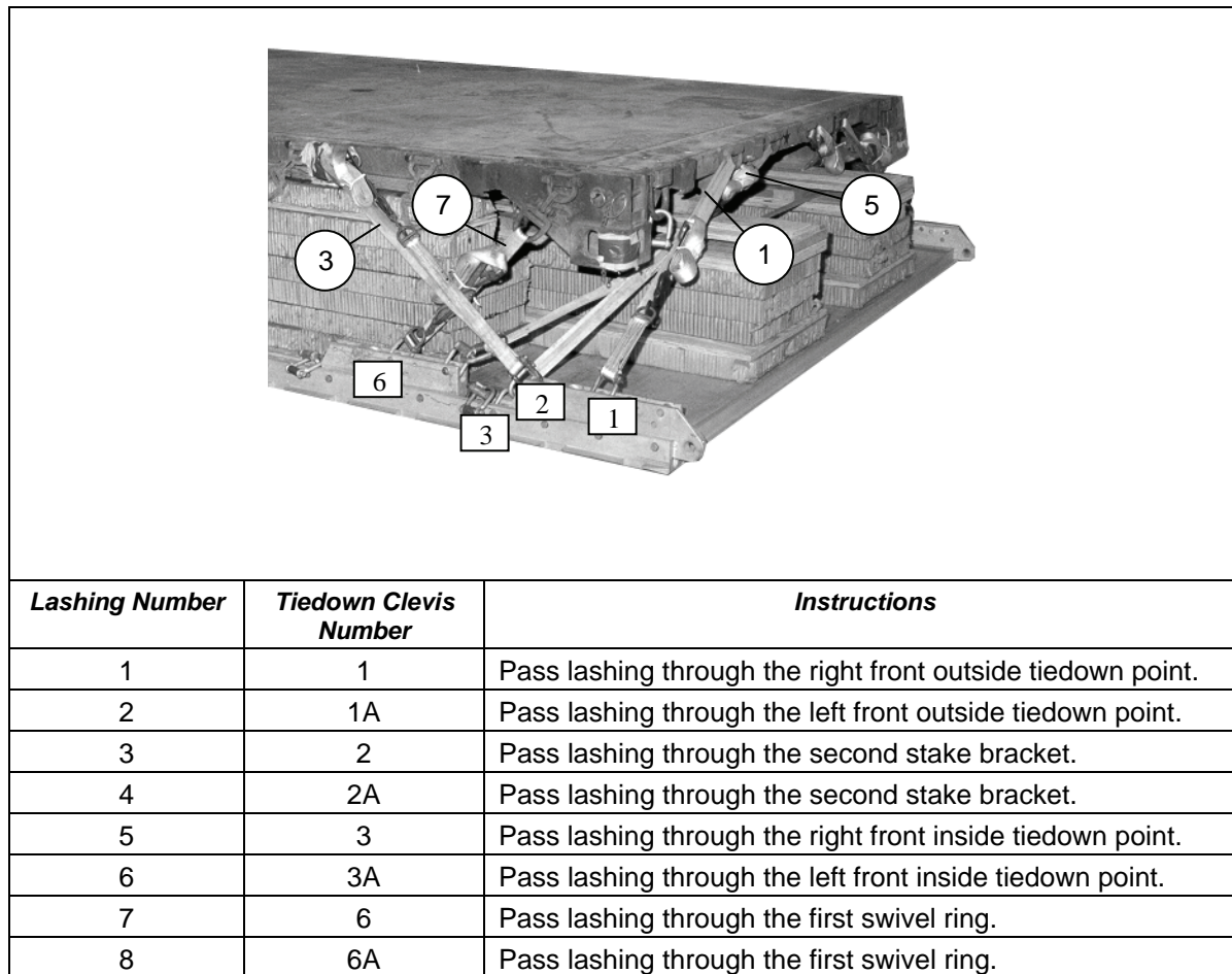
Figure 7-8. Pallet Lashed to Platform
