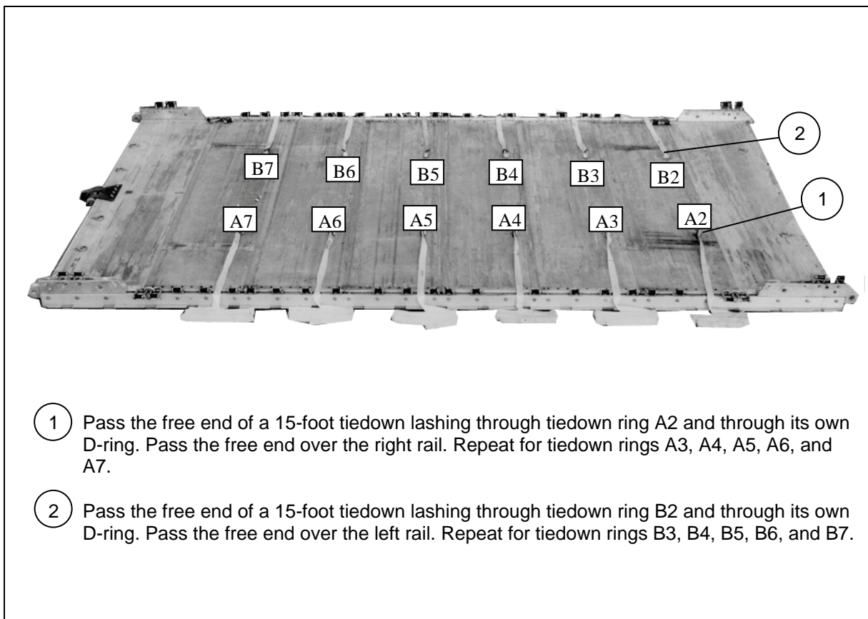
Figure 5-42. Lashings Pre-positioned on Platform
