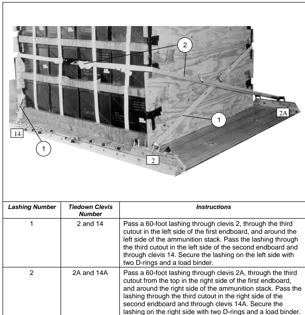
Figure 5-31. First Ammunition Stack and Endboards Lashed to Platform
