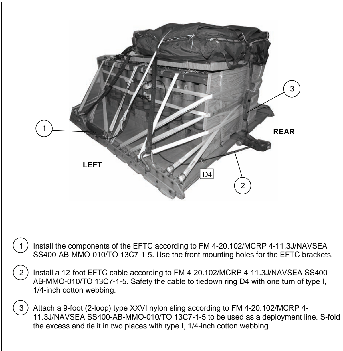
Figure 8-12. Extraction System Installed
