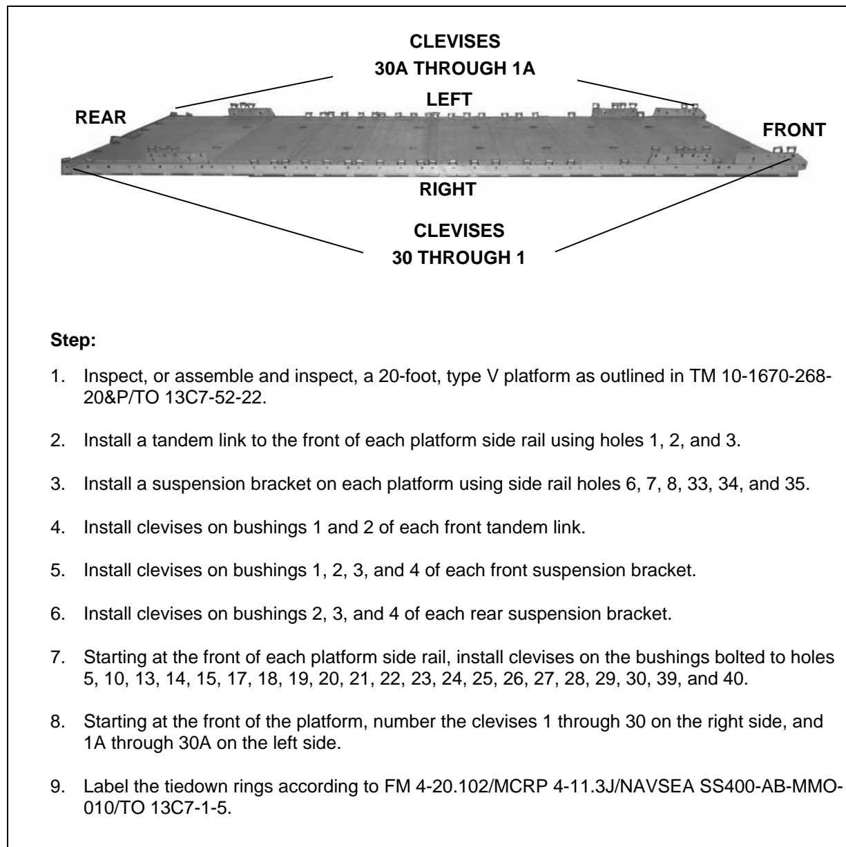
Figure 8-42. Platform Prepared
