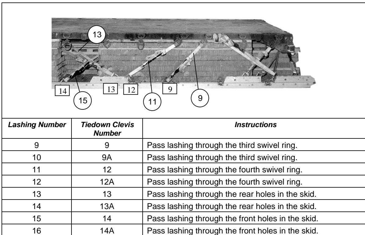
Figure 7-8. Pallet Lashed to Platform (Continued)
