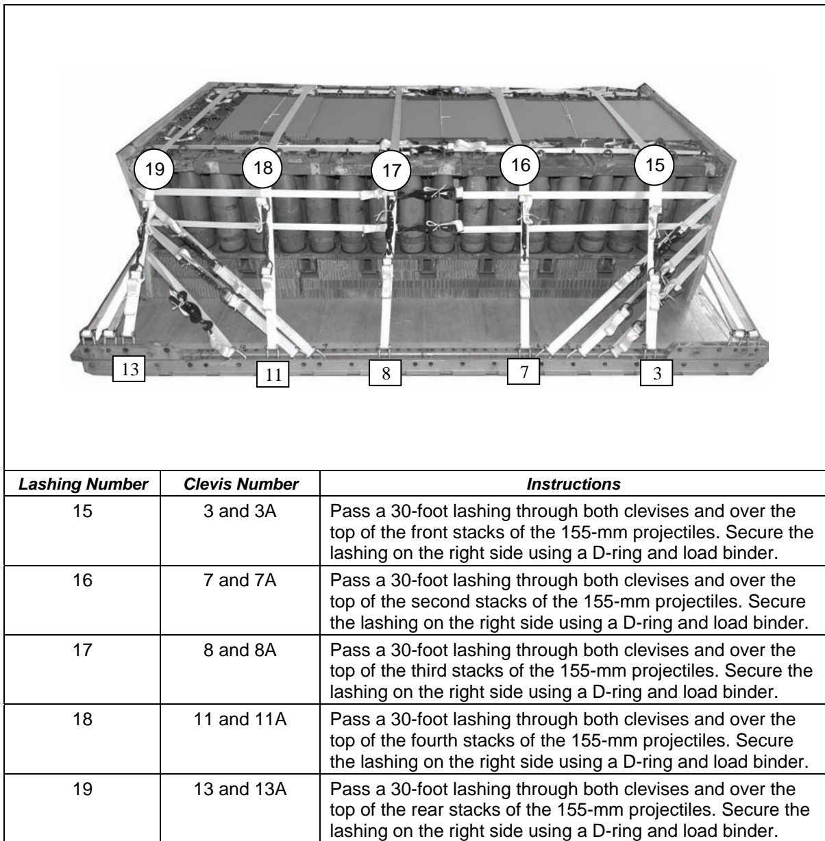
Figure 8-22. Ammunition Stack and Endboards Lashed (Continued)
