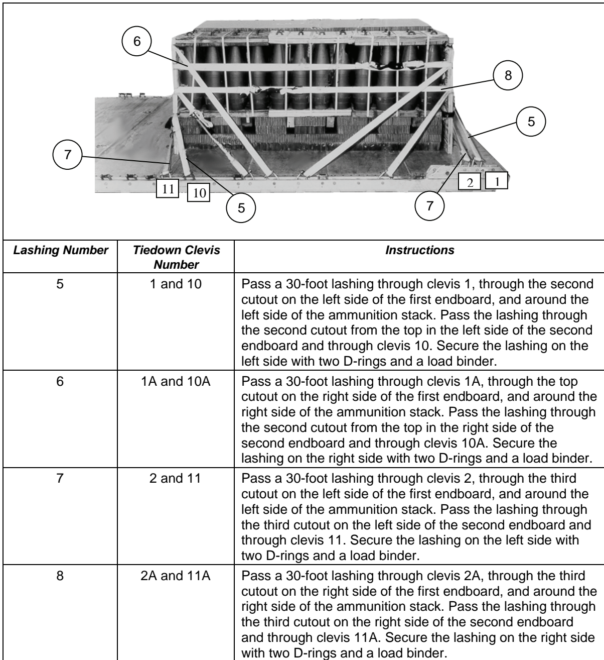
Figure 5-19. Lashings Installed for First Stack (Continued)
